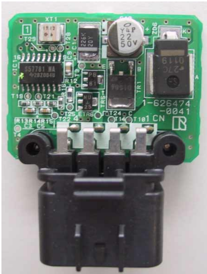
Printed Circuit Board for Amplifier (Top view)
