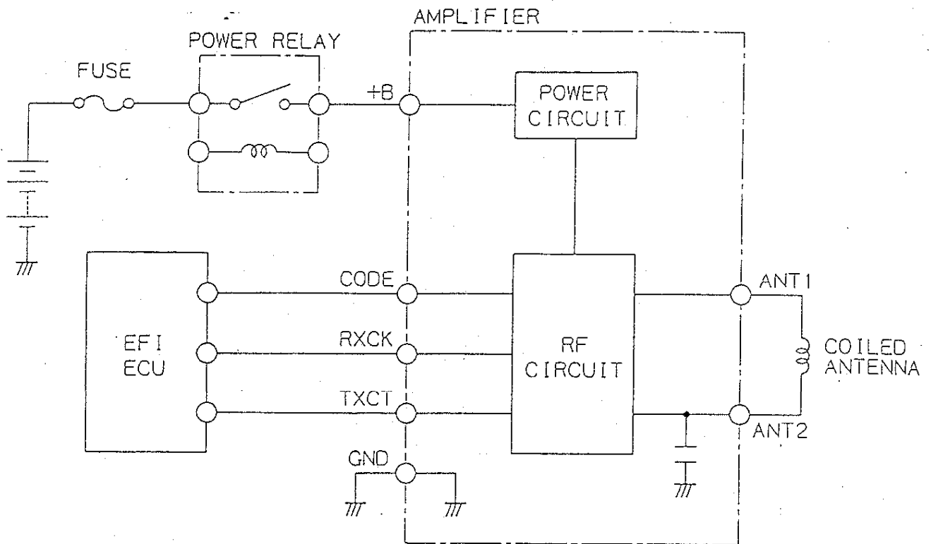
Block Diagram of Amplifier
