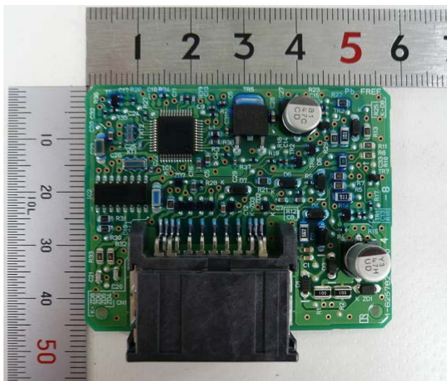
PC board (Front View)
