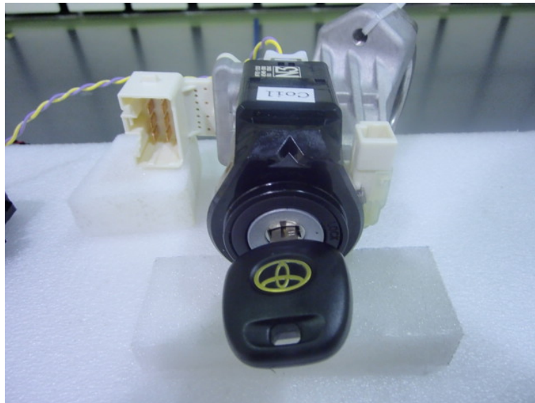
Mechanical Key (Inserted)
