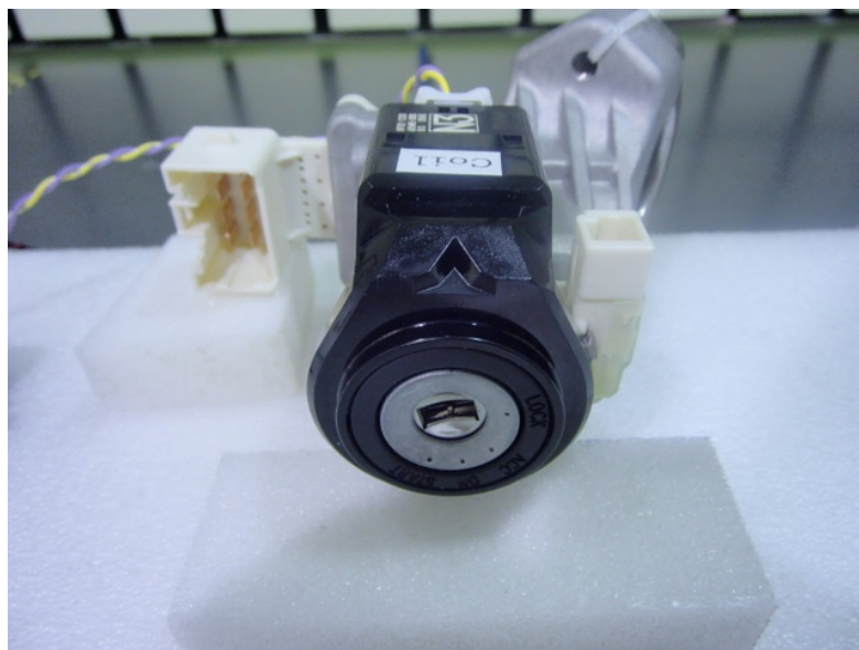
Mechanical Key (Not Inserted) Worst
