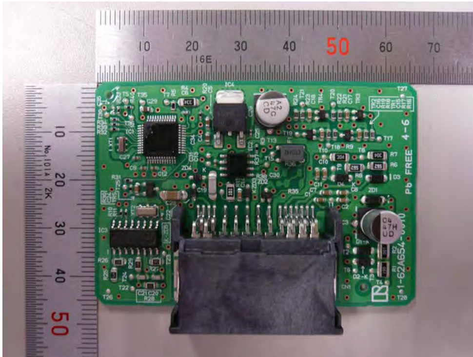
PC board (Reverse View)
