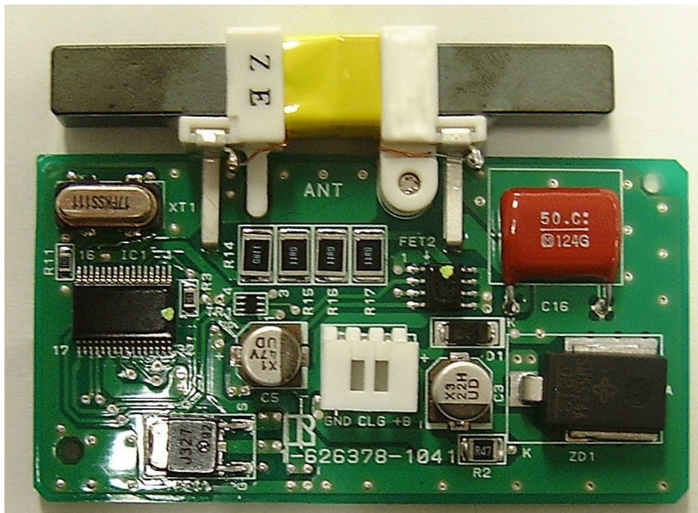
Room Oscillator MDL RO-2TY-1 Mother Board (Top view)
