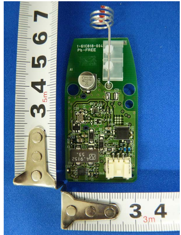
Rear View
