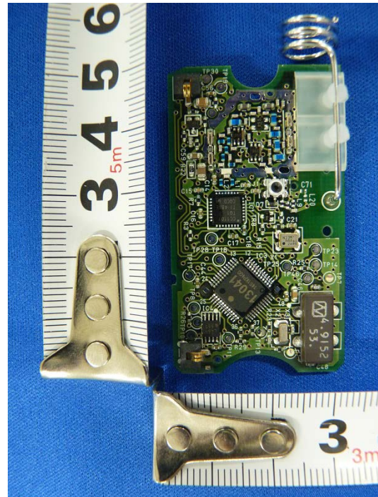
Reverse View
