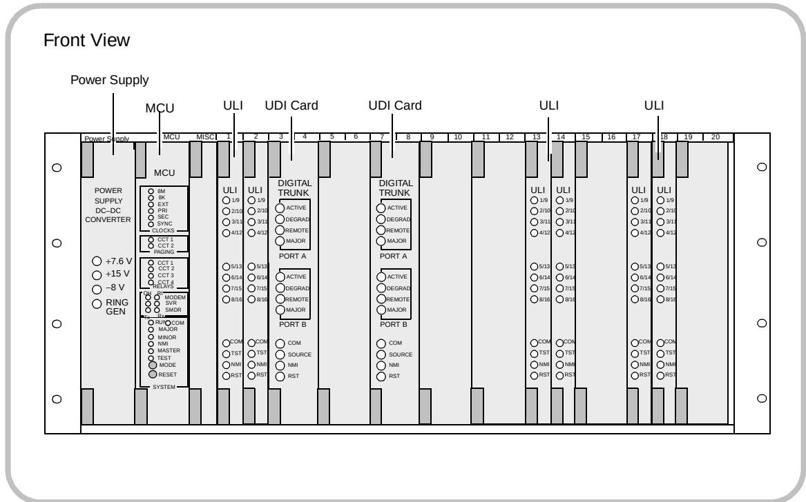
Figure 1-22 DMUX Shelf: 60 trunks (E1) with 96 Subscriber Lines
