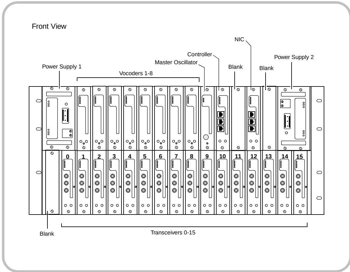
Figure 1–25 BTS Shelf
