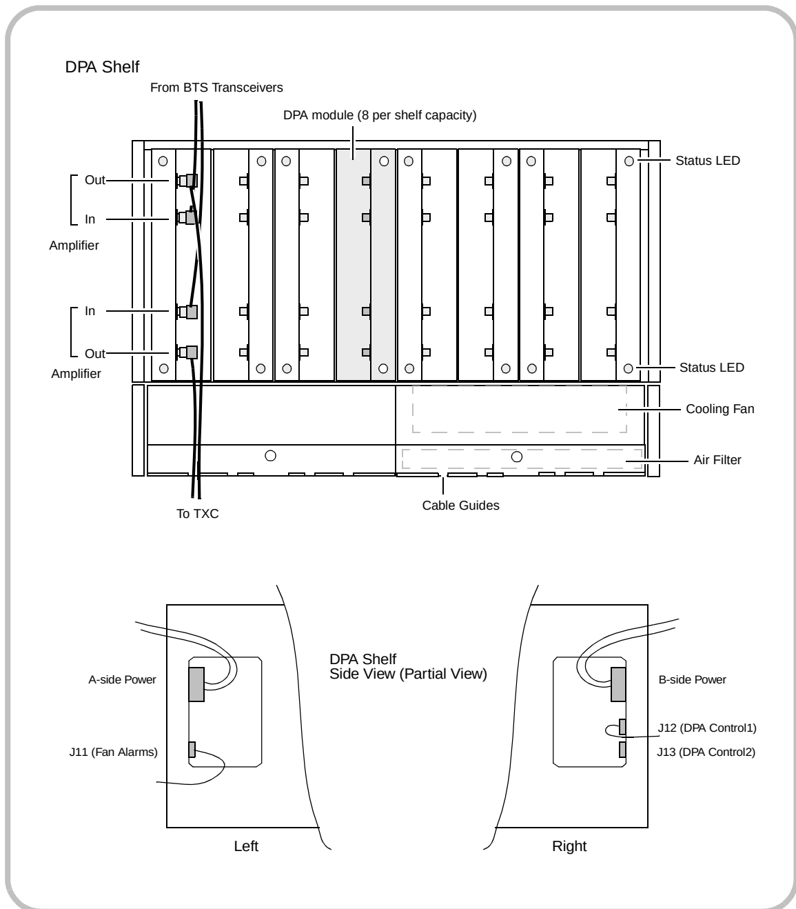
Figure 1–32 DPA Shelf
