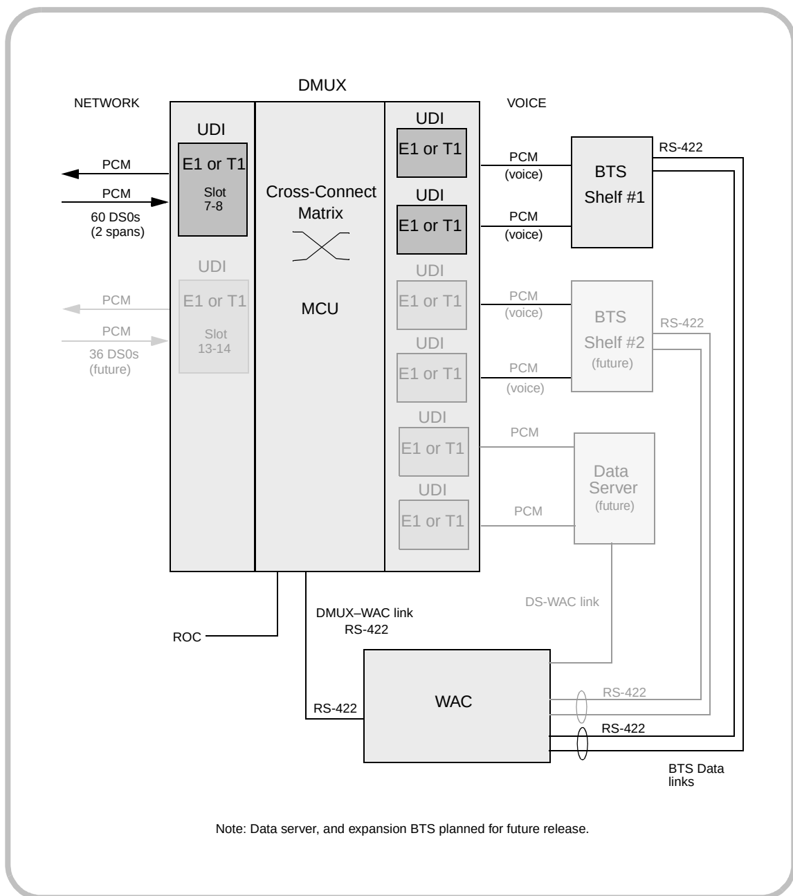
Figure 1-23 96-channel DMUX
