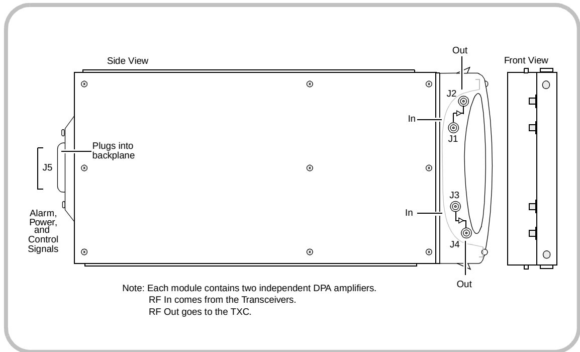
Figure 1–33 DPA Module
