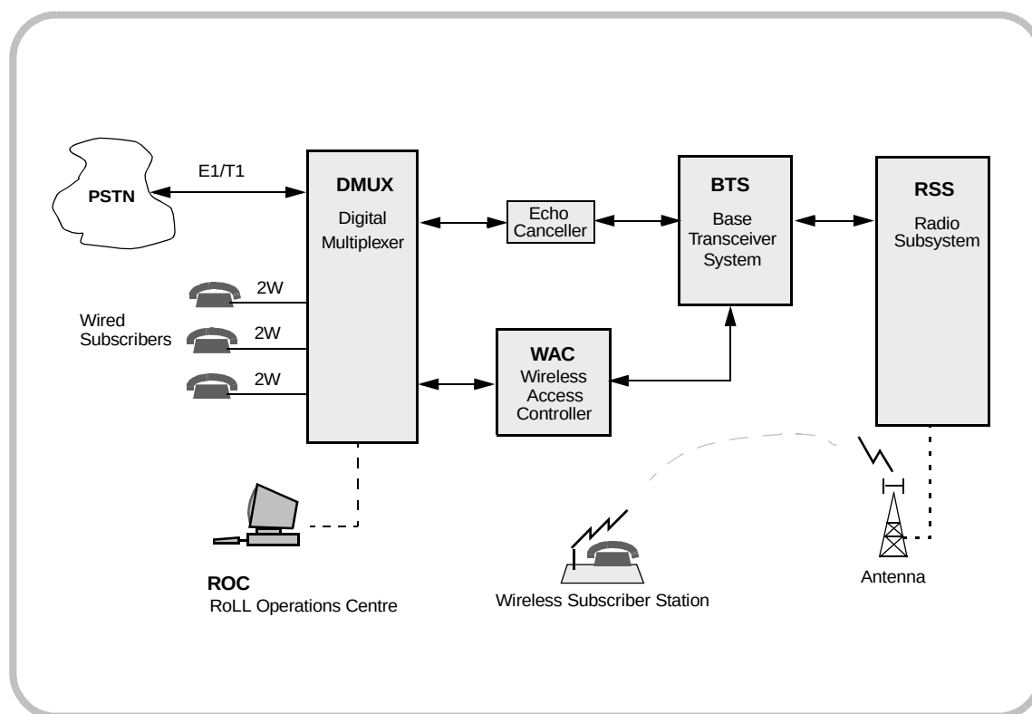
Figure 1–2 WINRoLL 136 Subsystems
