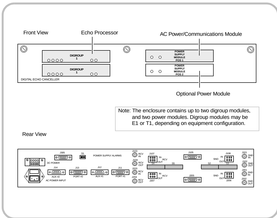
Figure 1–15 Echo Canceller
