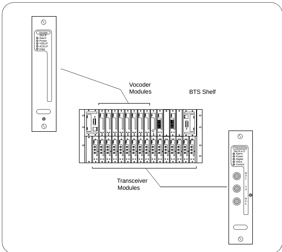
Figure 50 Optional BTS Transceiver and Vocoder Modules
