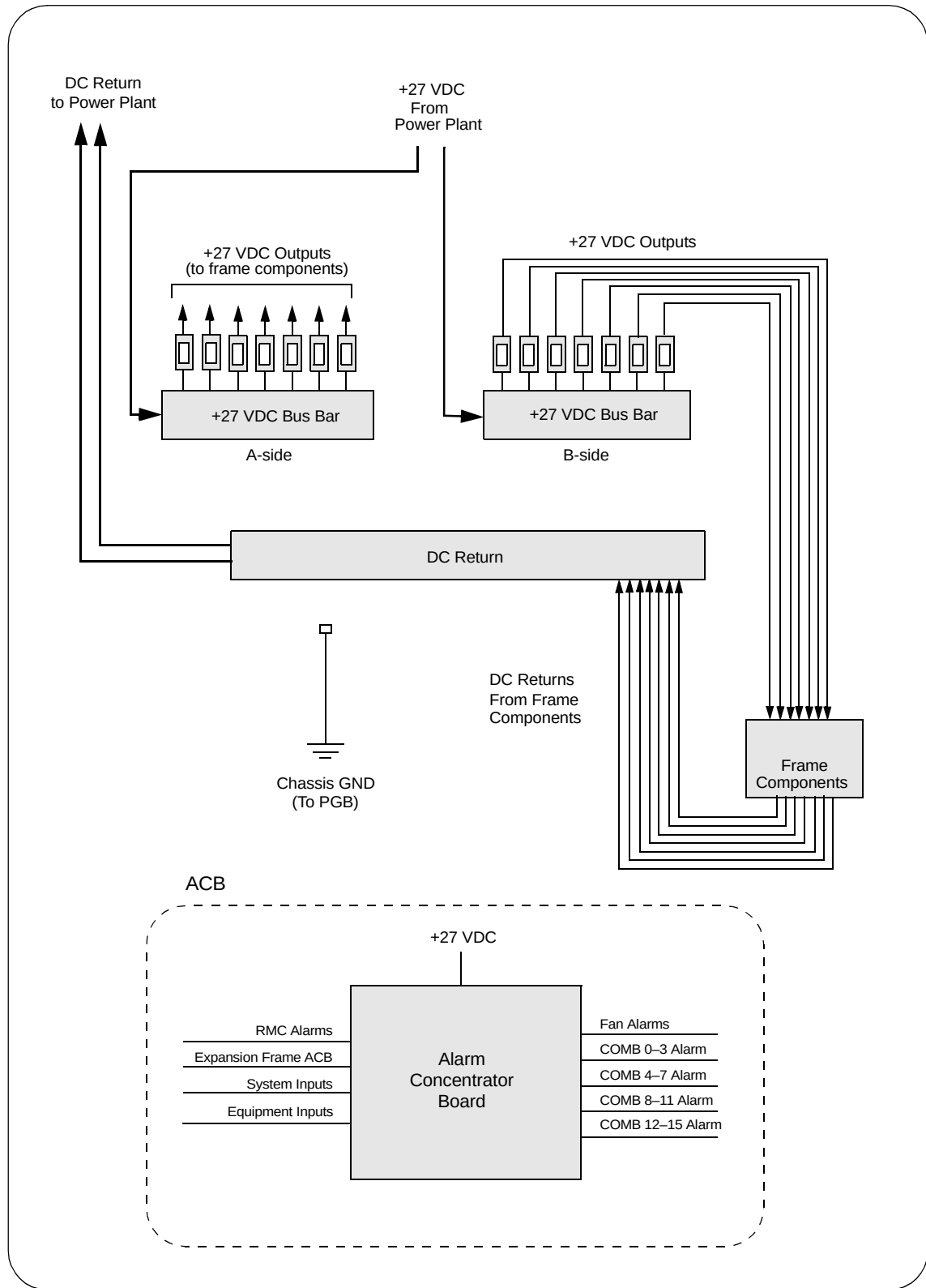
Figure 15 Power Distribution Shelf, Block Diagram
