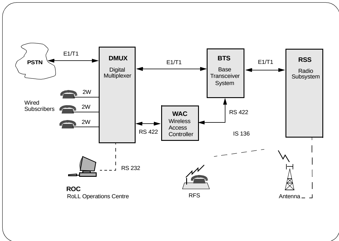
Figure 2 Subsystems
