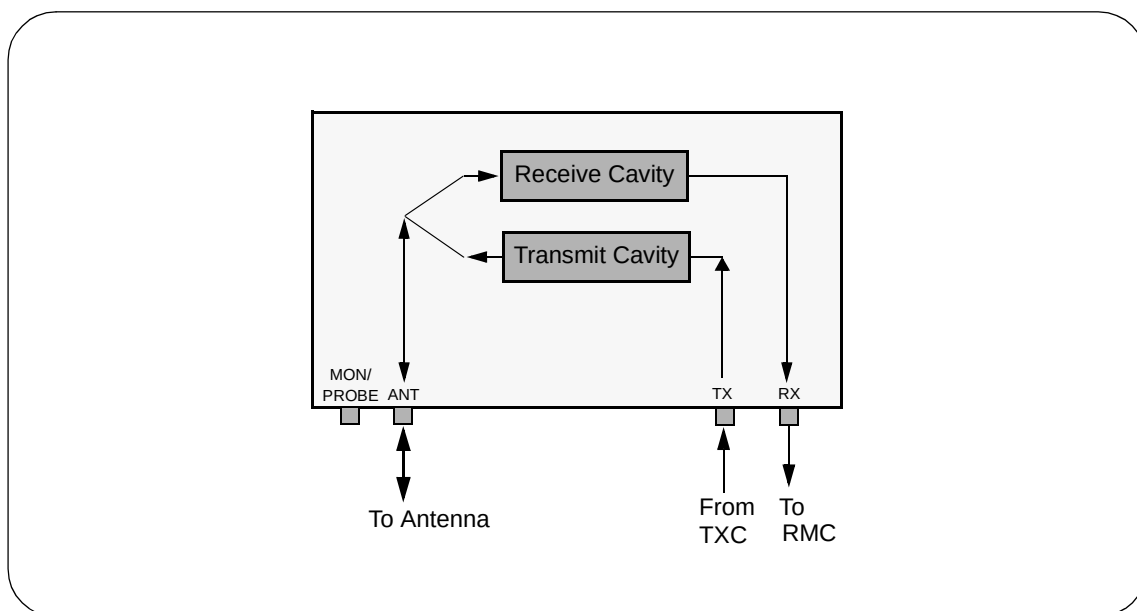
Figure 35 Duplexer Block Diagram
