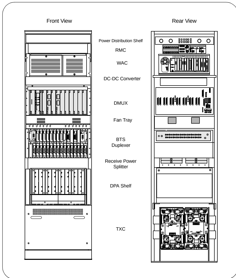
Figure 10 Main Components
