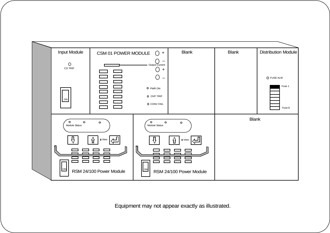
Figure 52 Power Supply Unit, Front View
