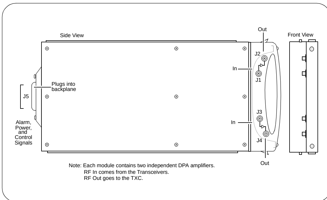
Figure 39 DPA Module
