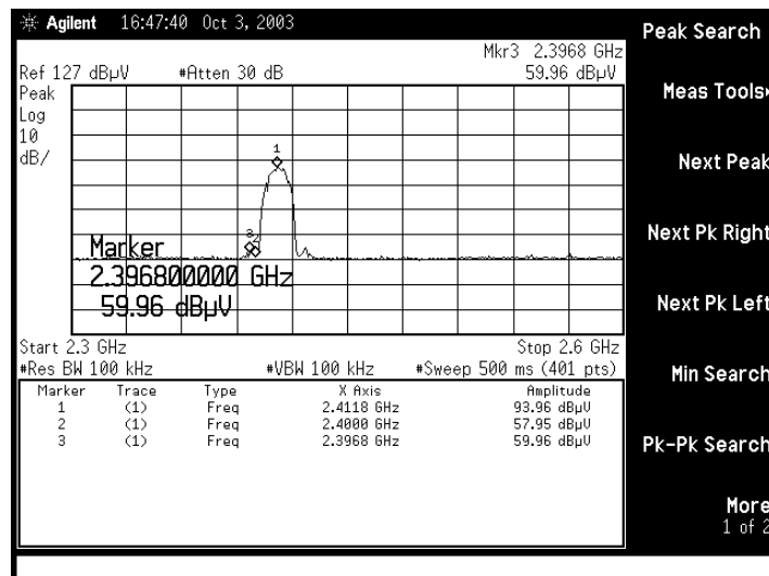
Figure Channel 1: (Horizontal)
