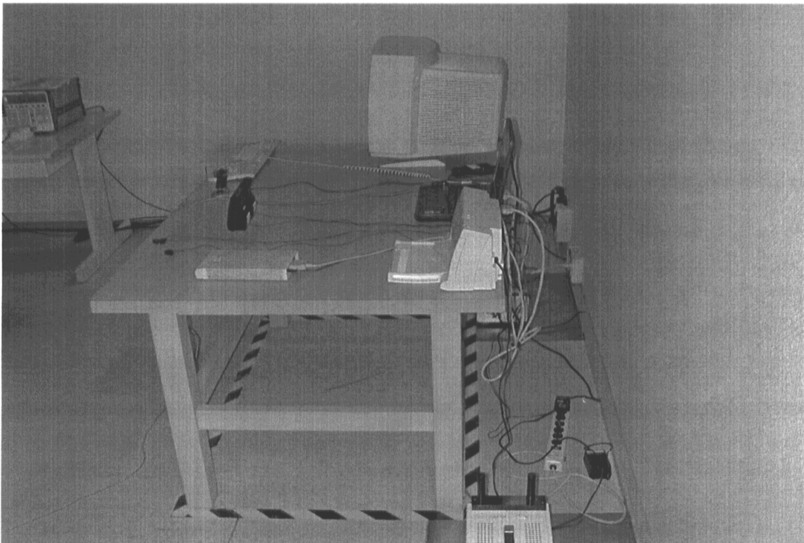
Back View of Conducted Test (Mode 2)
