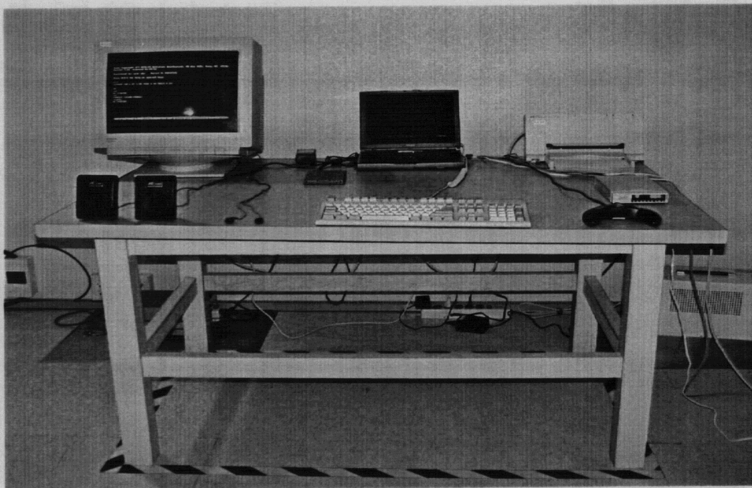
Mode 1 :Back View of Conducted Test ( Maximum Testing Configuration)
