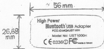
Bottom View
