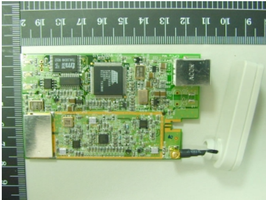
Photo 1: Inner view
