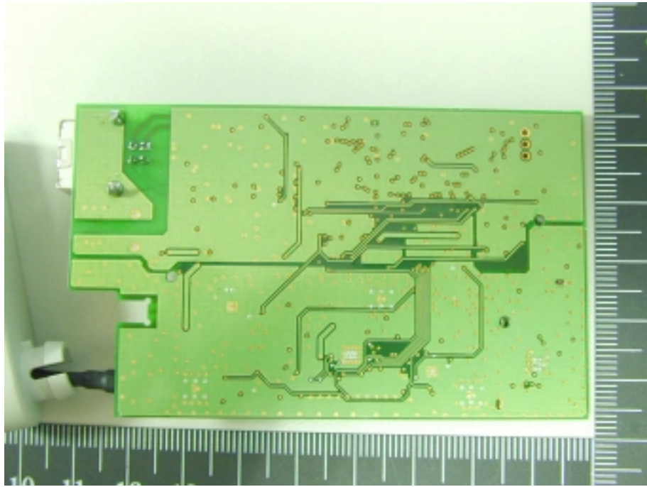
Photo 3: Inner view
