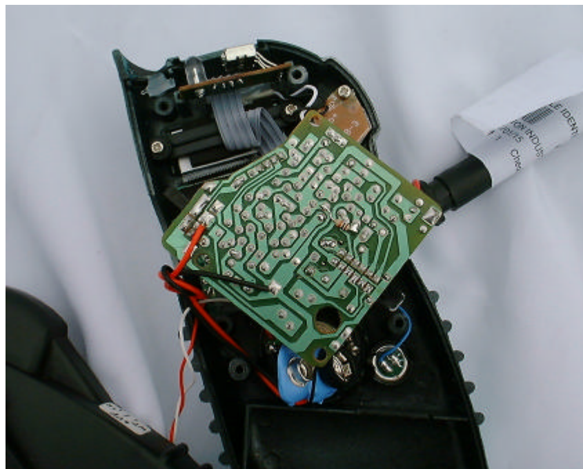
INNER CIRCUIT BOTTOM VIEW
