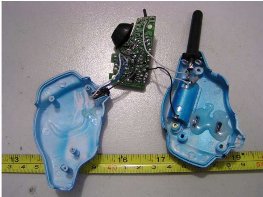
EUT – Uncovered View (2)
