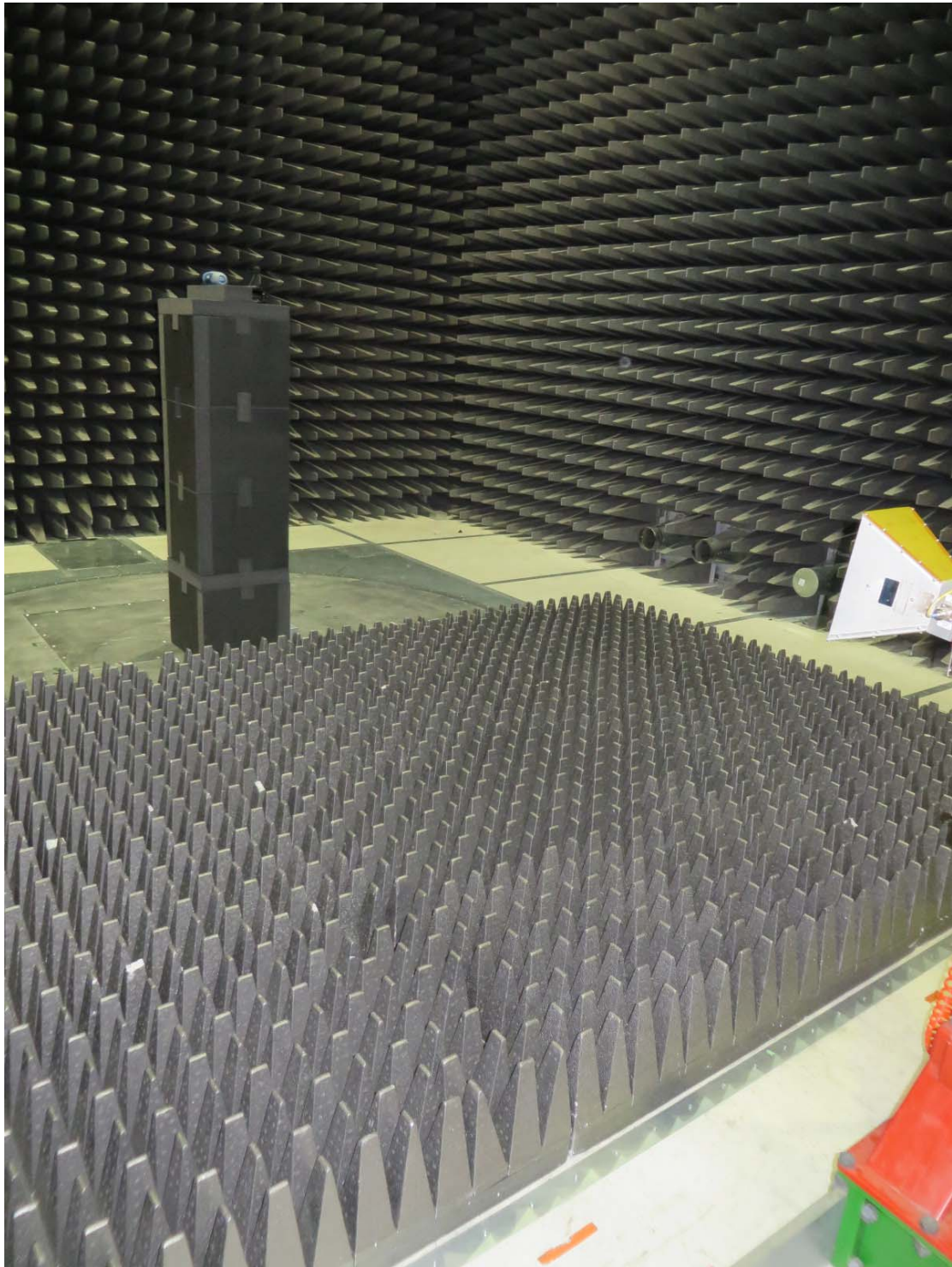
Transmit Mode Above 1 GHz
