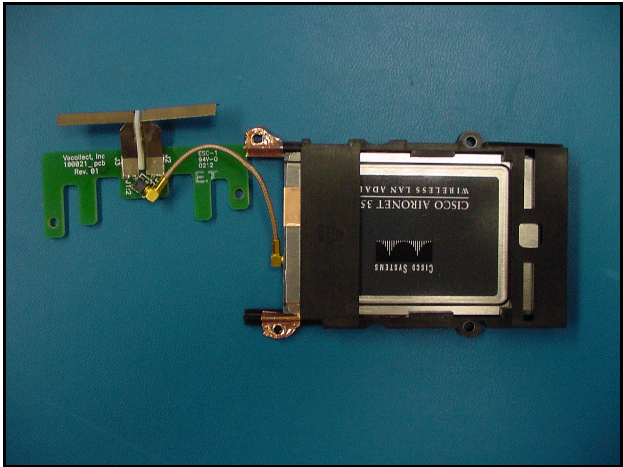
PHOTOGRAPH 20: WLAN CARD FRONT WITH ANTENNA
