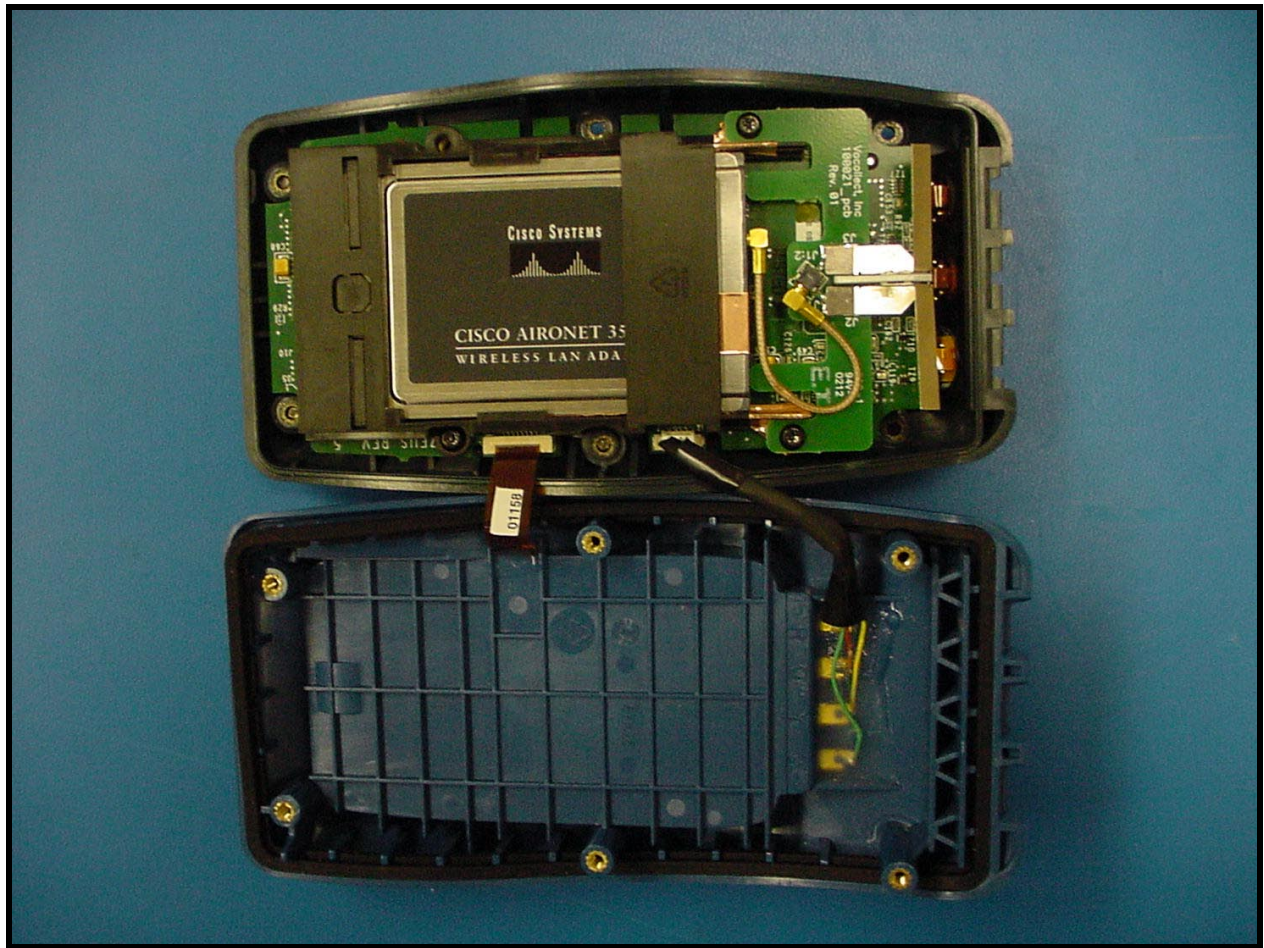
PHOTOGRAPH 14: INTERNAL VIEW WITH WLAN CARD
