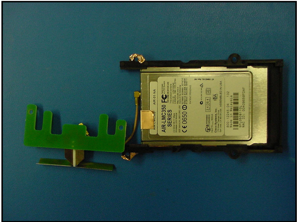
PHOTOGRAPH 21: WLAN CARD REAR WITH ANTENNA
