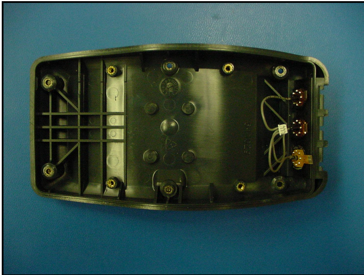
PHOTOGRAPH 16: INSIDE REAR COVER
