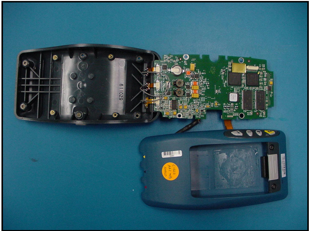
PHOTOGRAPH 12: OVERALL INTERNAL VIEW, REAR VIEW OF PCB
