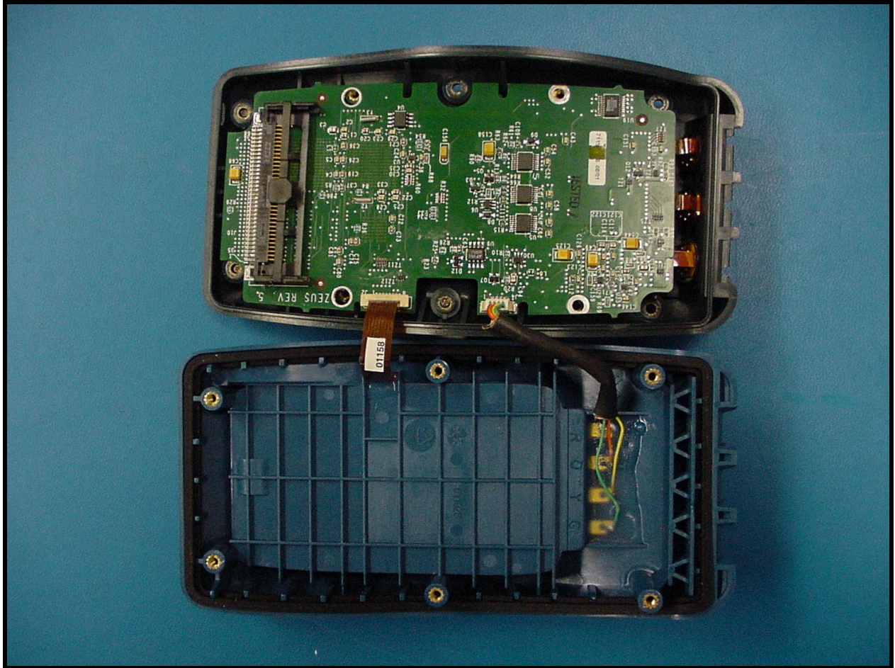
PHOTOGRAPH 11: OVERALL INTERNAL VIEW
