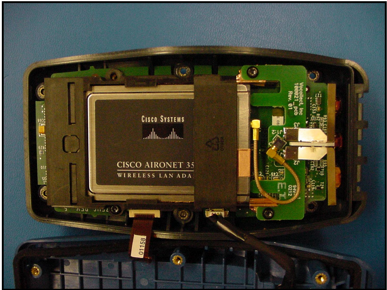
PHOTOGRAPH 13: INTERNAL VIEW WITH WLAN CARD
