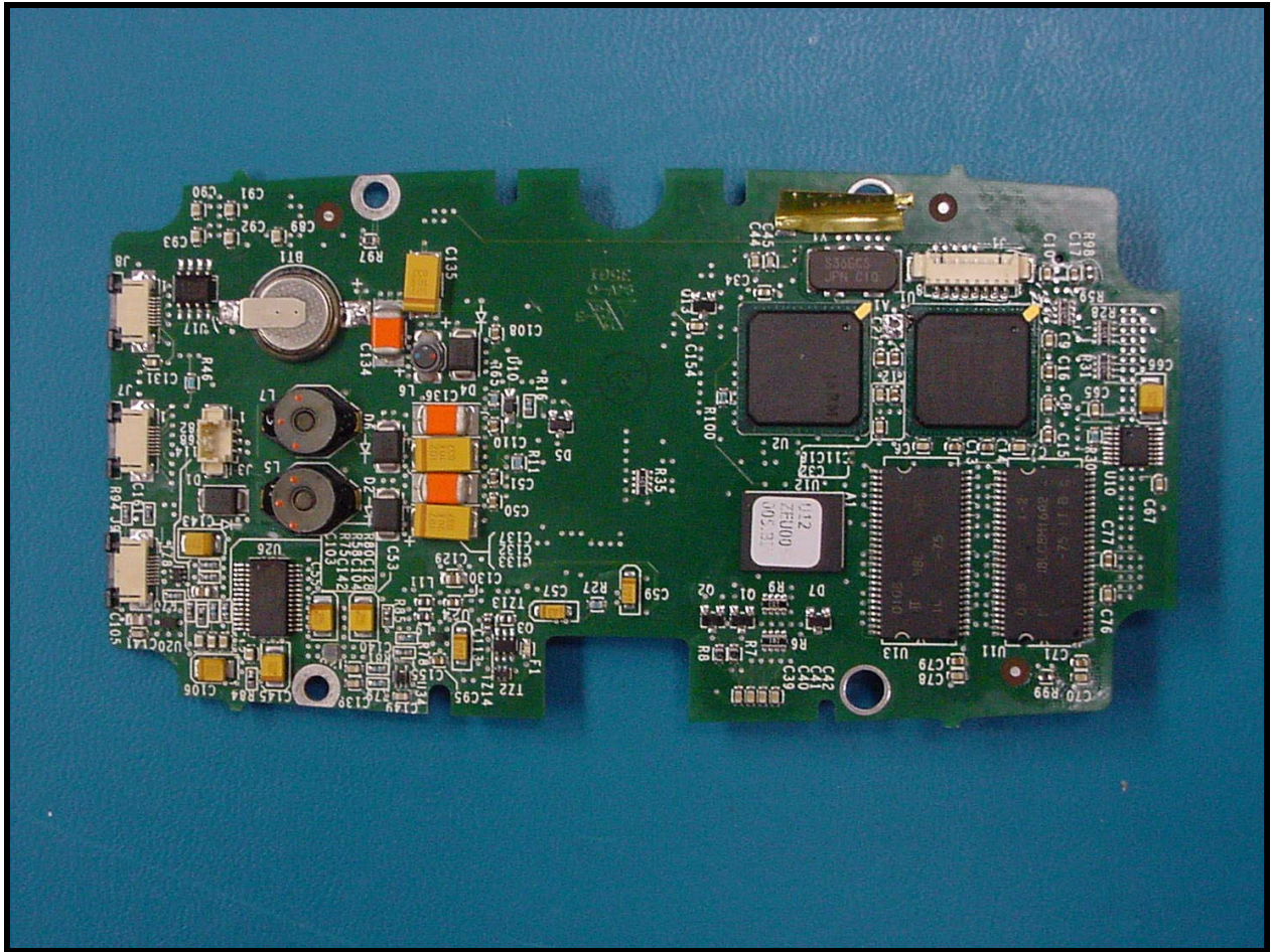
PHOTOGRAPH 19: PCB REAR WITHOUT SHIELD
