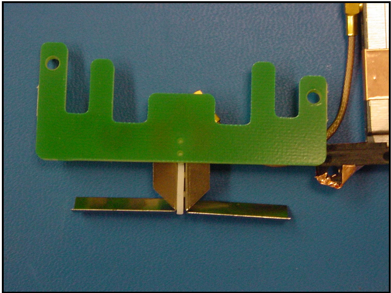
PHOTOGRAPH 23: ANTENNA REAR
