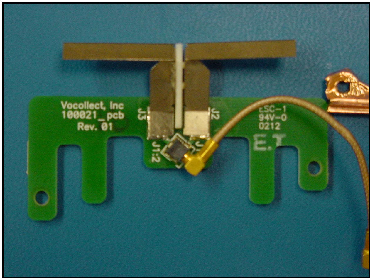
PHOTOGRAPH 22: ANTENNA FRONT
