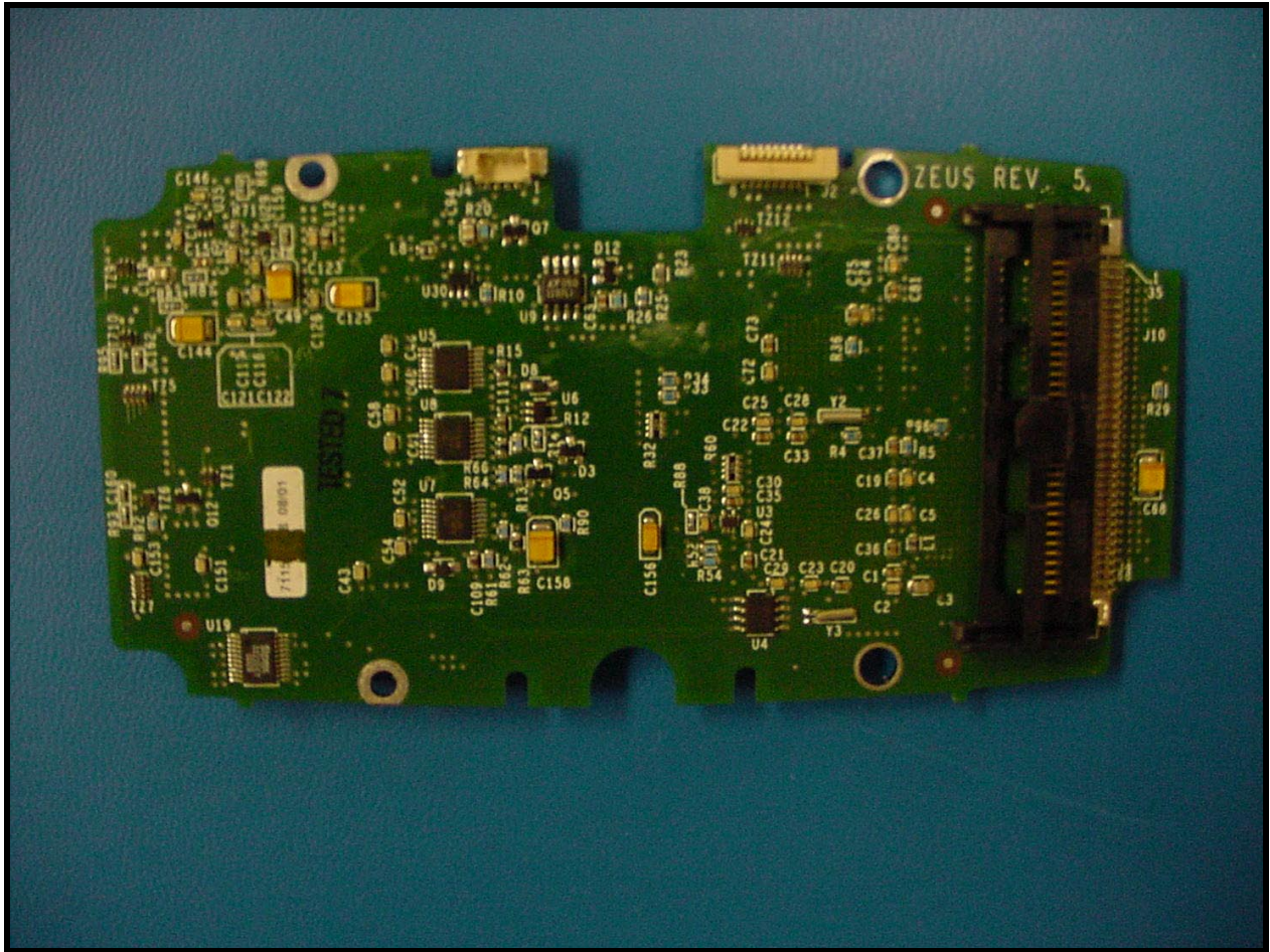
PHOTOGRAPH 17: PCB FRONT
