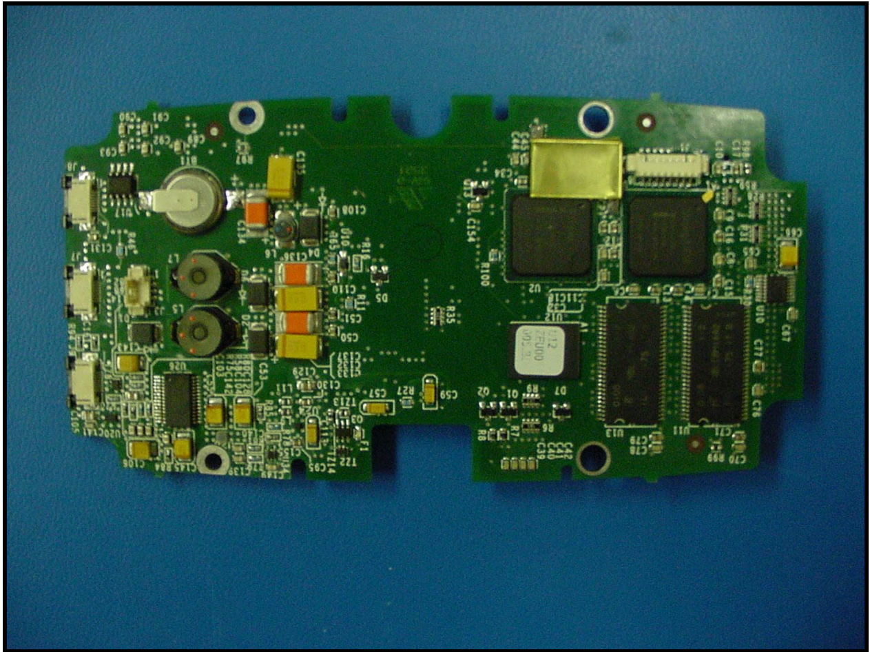
PHOTOGRAPH 18: PCB REAR WITH SHIELD
