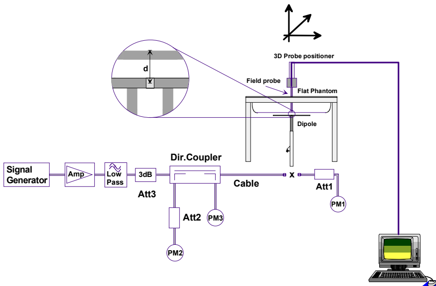
Figure 1. System Performance Check Measurement Setup
