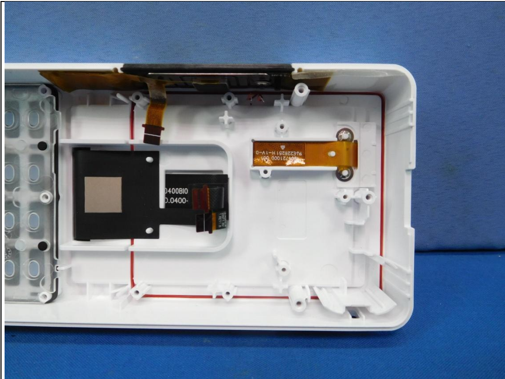
Antenna (Brand: XAC; Model: ASM T103P)
