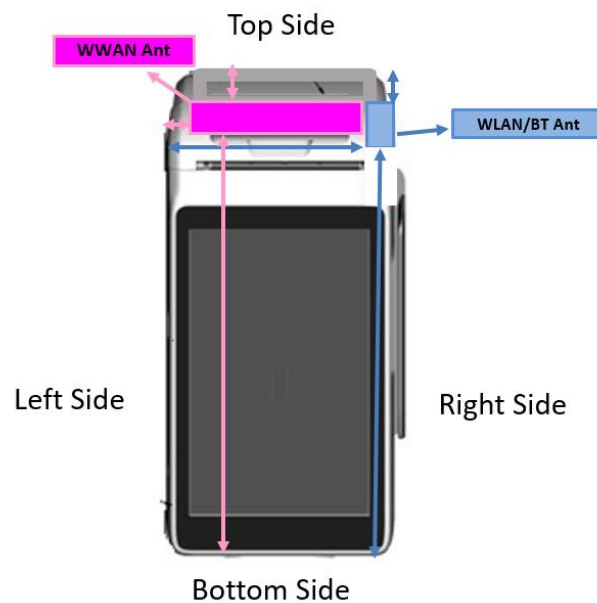
<EUT Front Face View>
