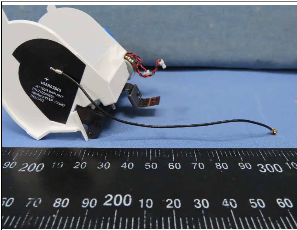
ANT1 (WLAN/Bluetooth)
