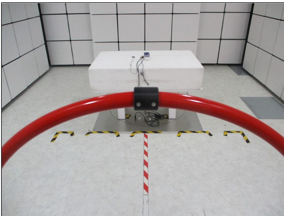
Loop Antenna
