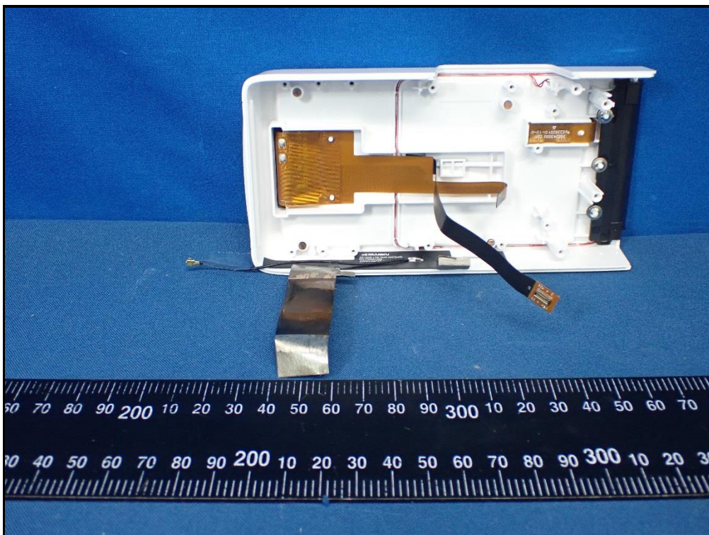
Antenna- WWAN-Aux
