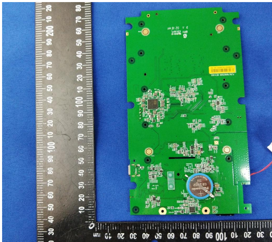
MAIN BOARD REAR VIEW
