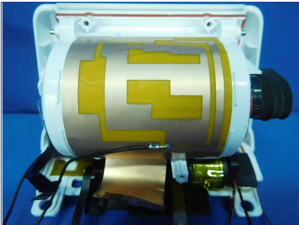
3G/LTE Antenna (Main)
