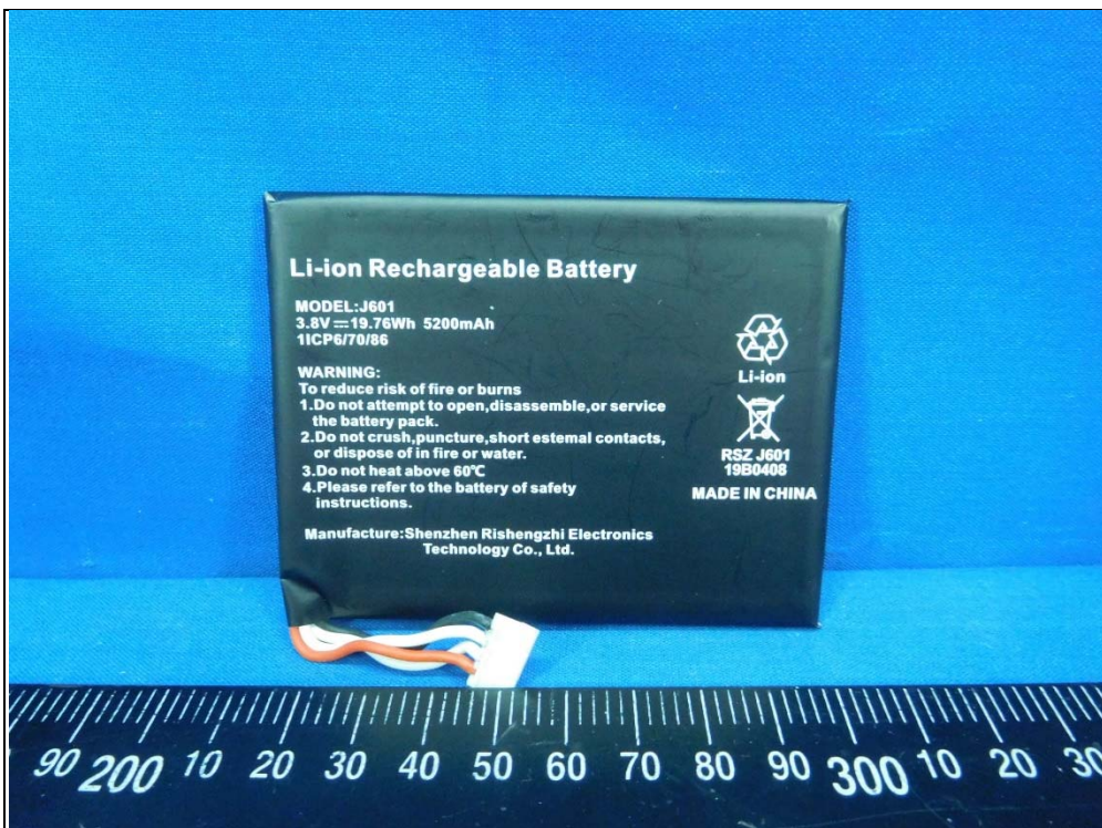
Battery (option)
