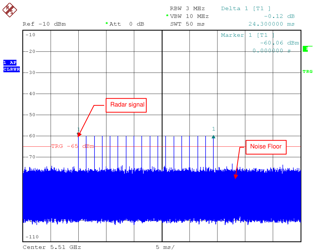
Radar Signal 0
