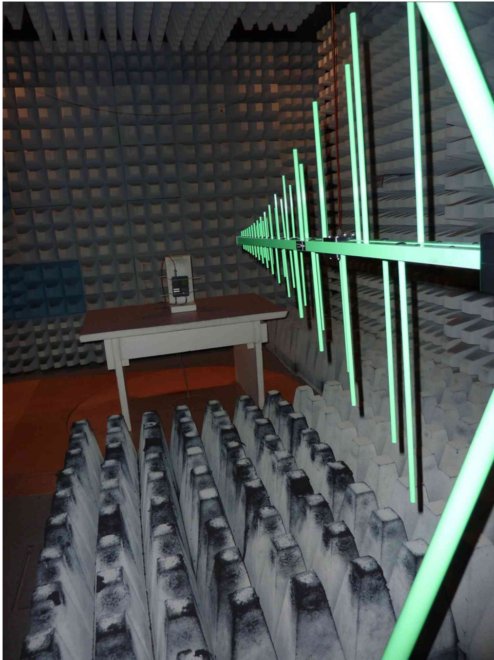
160575_02.JPG: Test setup - Radiated emission (fully anechoic chamber)
