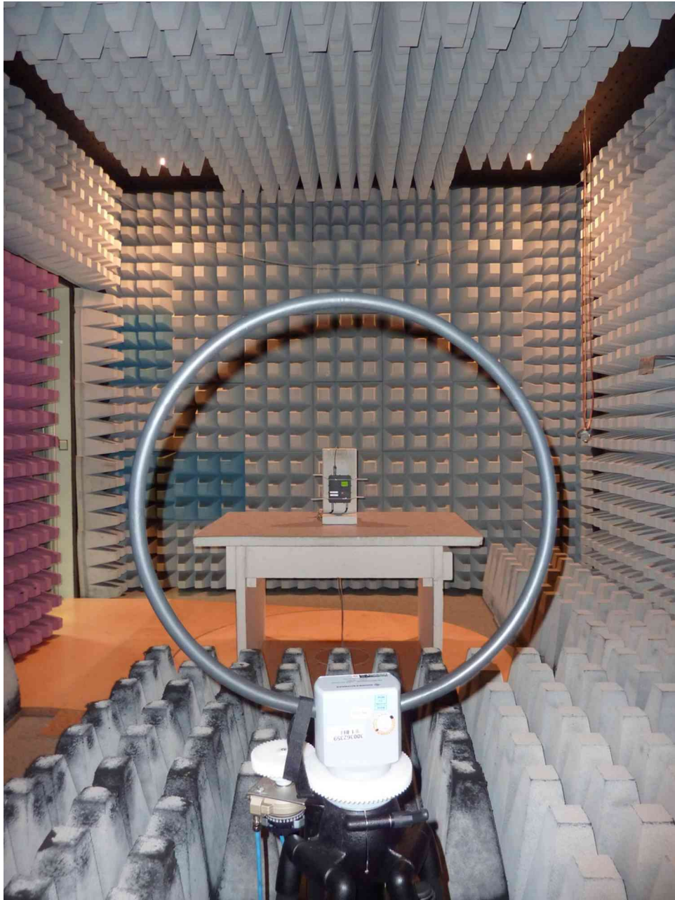
160575_01.JPG: Test setup - Radiated emission (fully anechoic chamber)
