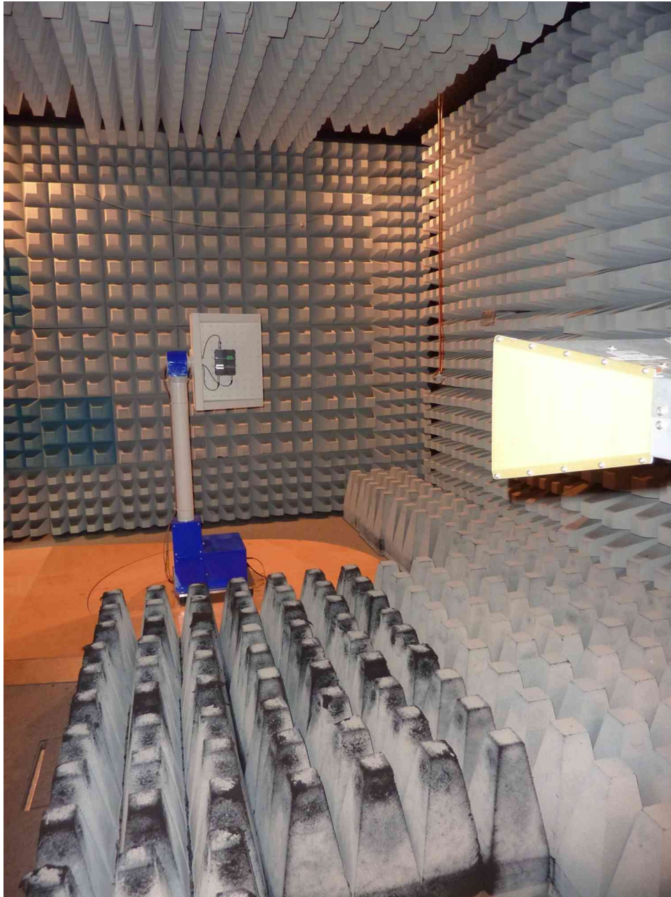
160575_03.JPG: Test setup - Radiated emission (fully anechoic chamber)
