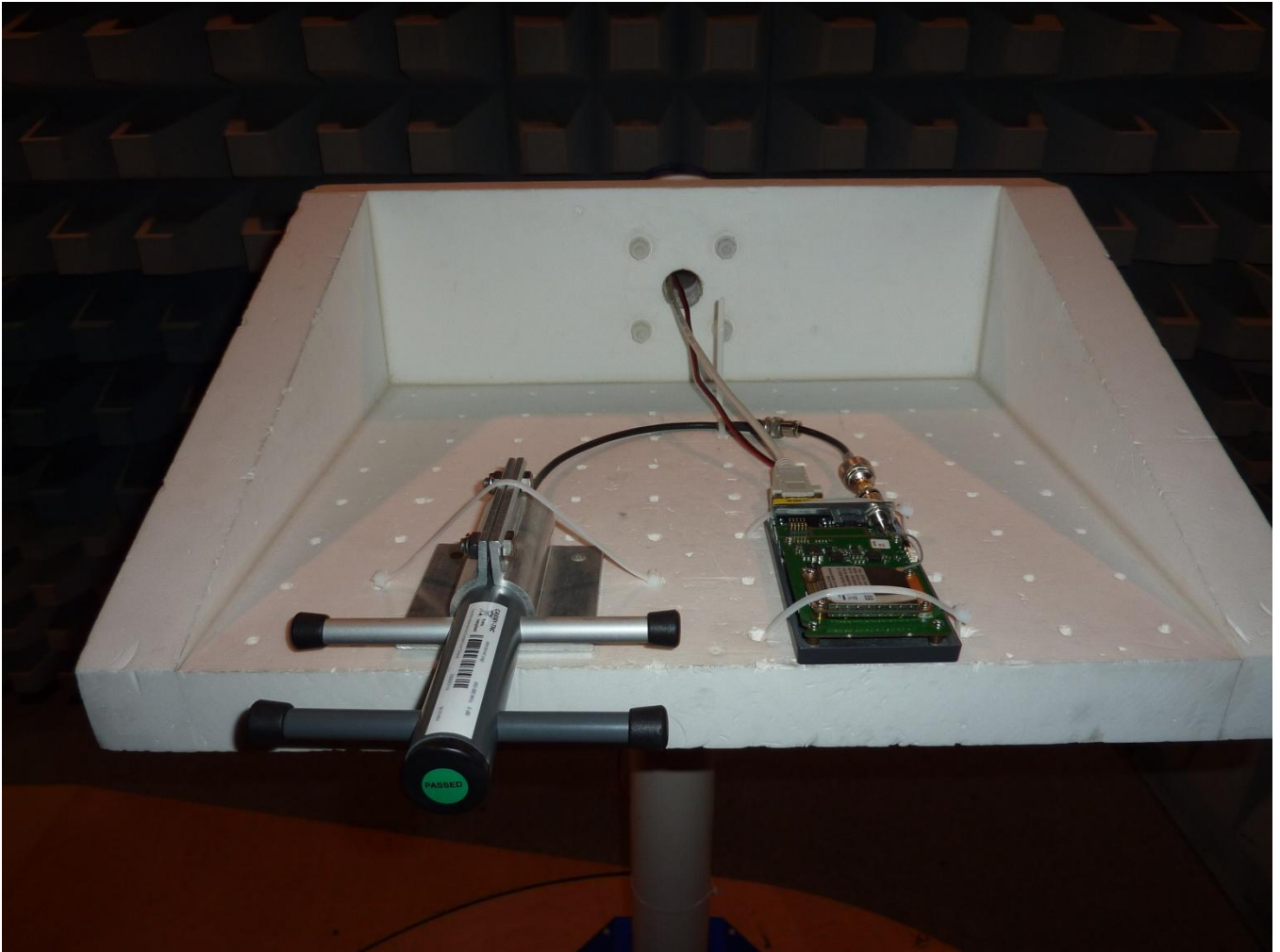
172629_21.JPG: Test setup CA930Y antenna - Radiated emission (fully anechoic chamber)
