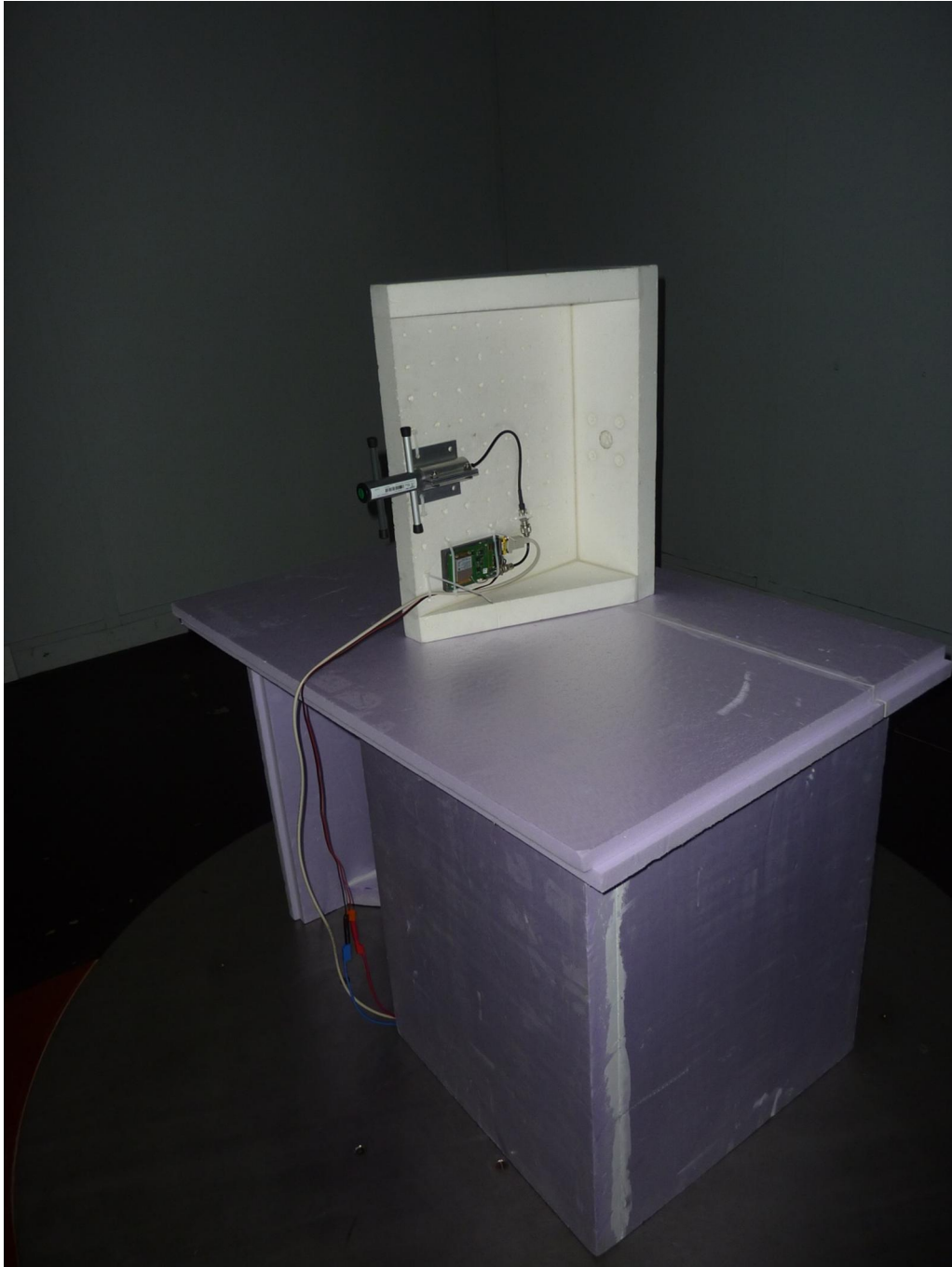
172629_23.JPG: Test setup CA930Y antenna - Radiated emission (OATS)
