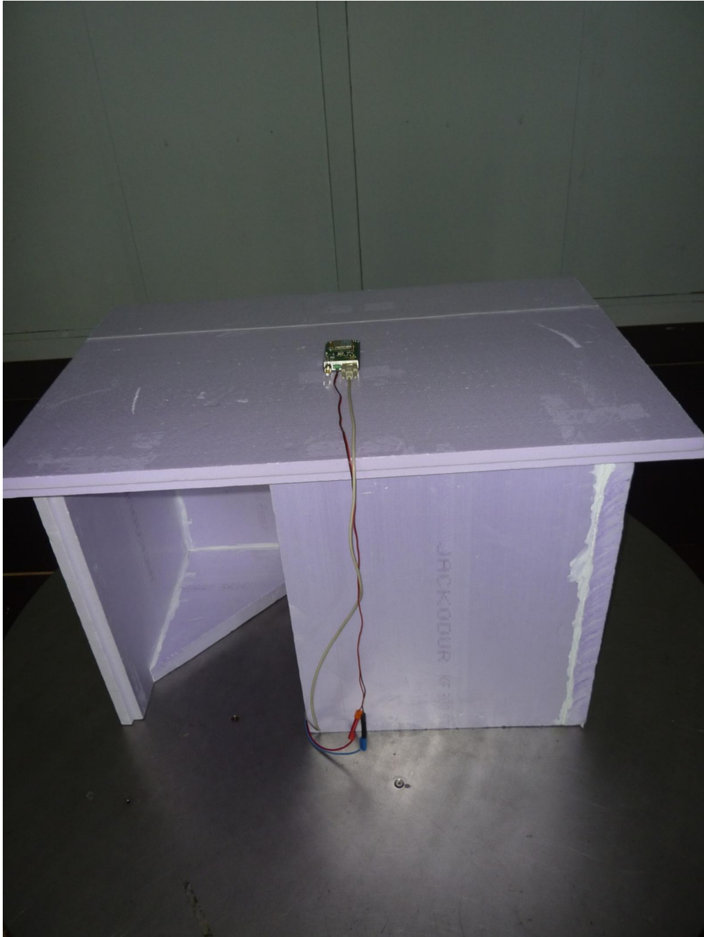
172629_03.JPG: Test setup antenna port terminated - Radiated emission (OATS)
