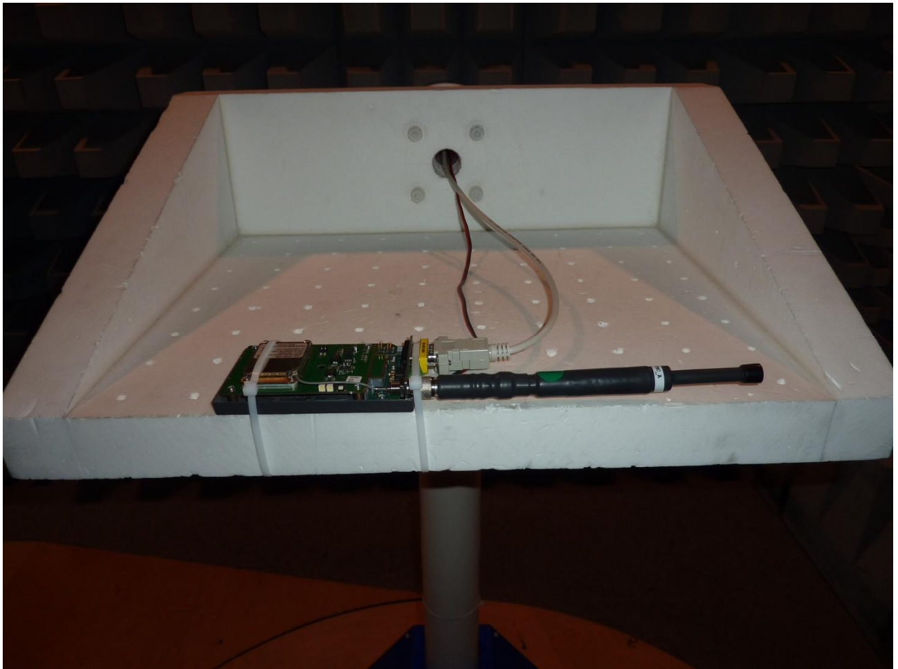
172629_20.JPG: Test setup CA915H antenna - Radiated emission (fully anechoic chamber)
