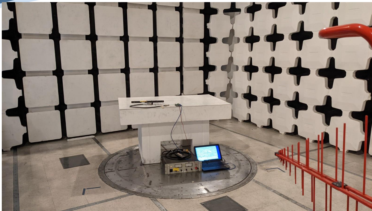
Transmitter Spurious Yagi Antenna Below 1GHz
