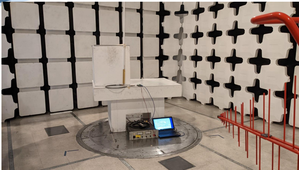
Transmitter Spurious Whip Antenna Below 1GHz
