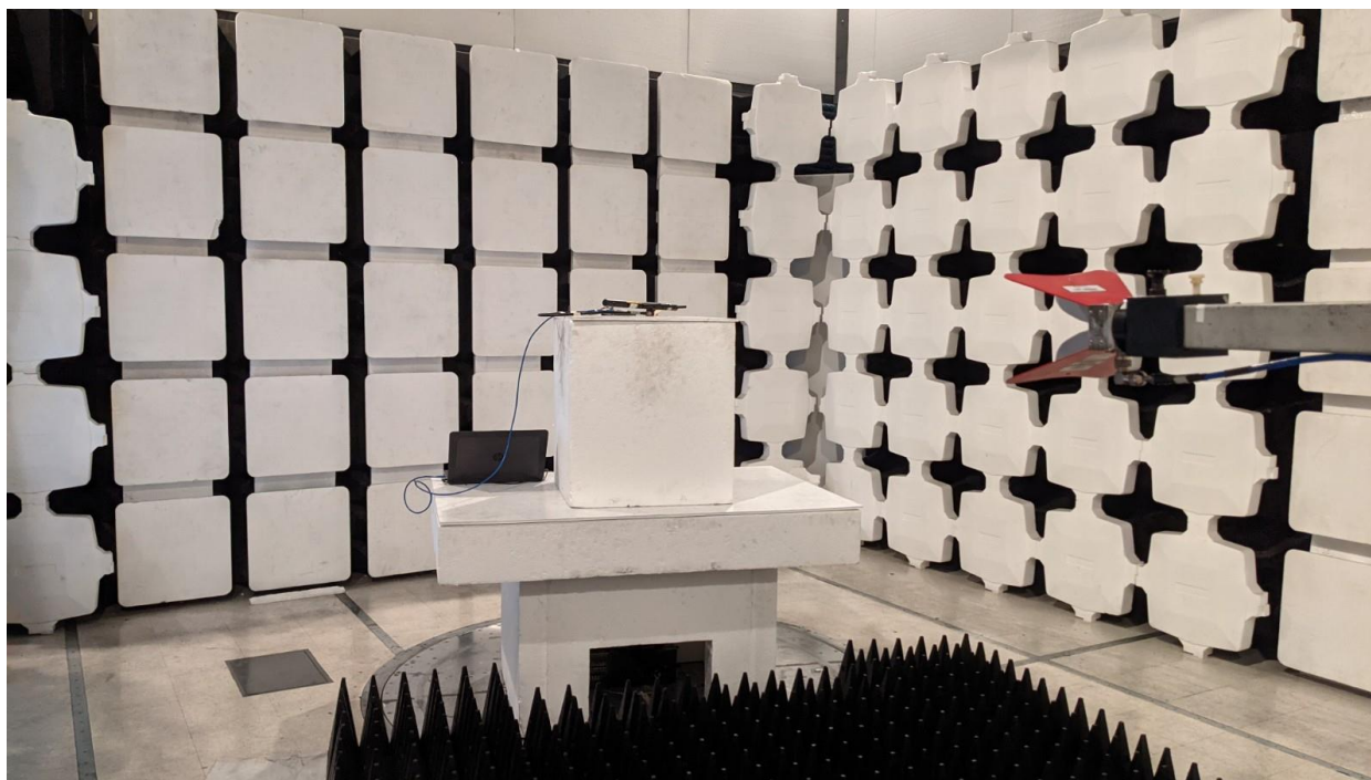
Transmitter Spurious Yagi Antenna Above 1GHz
