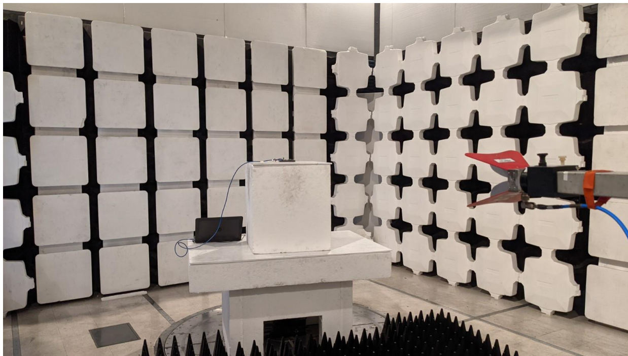
Transmitter Spurious 410-470 Above 1GHz
