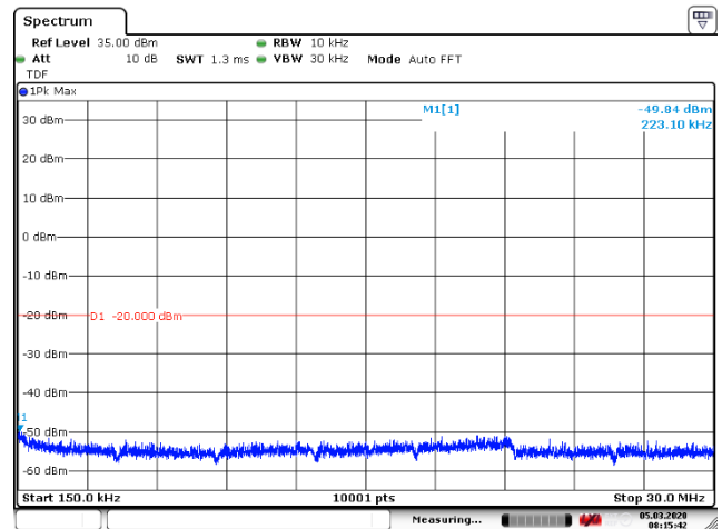
Figure 79: 150 kHz – 30 MHz
