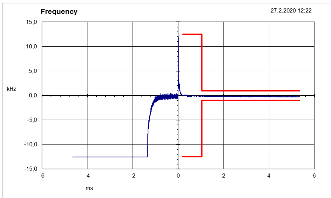
Figure 169: 429.5 MHz
