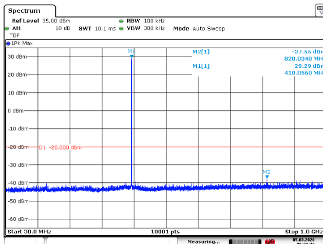
Figure 56: 30 – 1000 MHz
