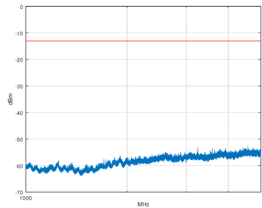
Figure 163: 469.5 MHz, X-orientation
