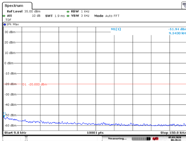
Figure 82: 9 – 150 kHz
