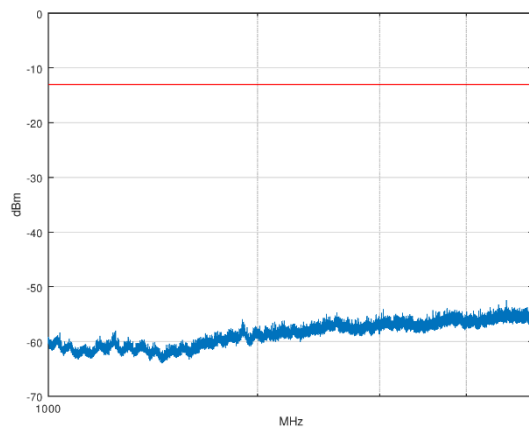
Figure 162: 450.5 MHz, Z-orientation
