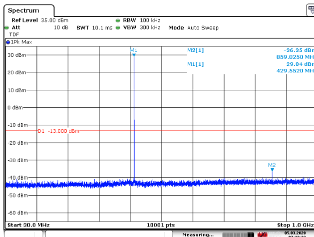
Figure 112: 30 – 1000 MHz
