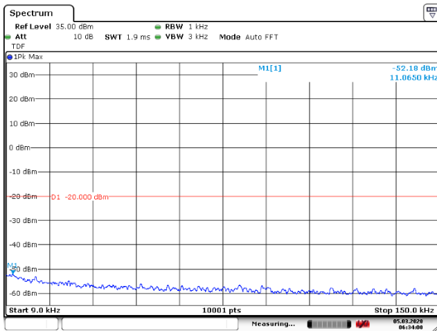
Figure 58: 9 – 150 kHz
