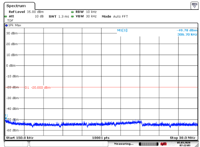
Figure 67: 150 kHz – 30 MHz
