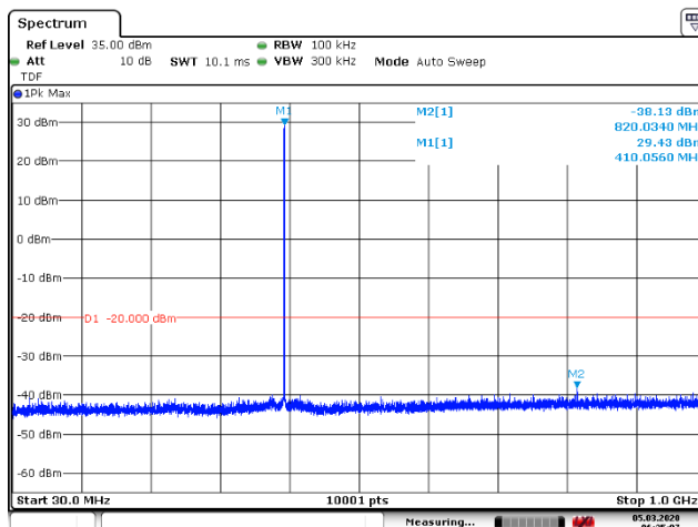
Figure 52: 30 – 1000 MHz
