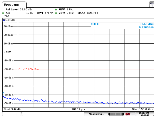
Figure 78: 9 – 150 kHz
