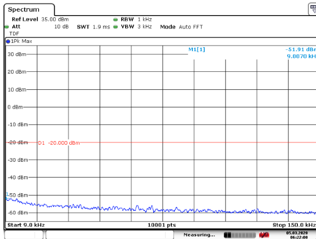
Figure 50: 9 – 150 kHz
