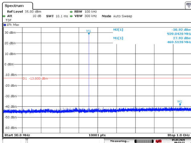
Figure 144: 30 – 1000 MHz
