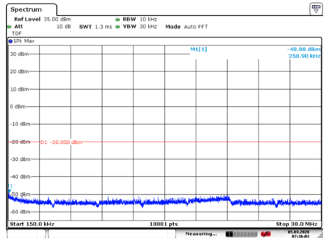
Figure 71: 150 kHz – 30 MHz
