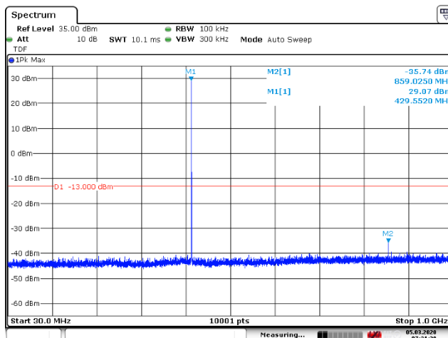
Figure 120: 30 – 1000 MHz
