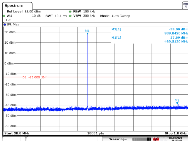
Figure 140: 30 – 1000 MHz
