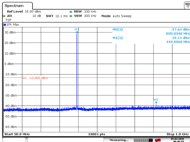
Figure 100: 30 – 1000 MHz
