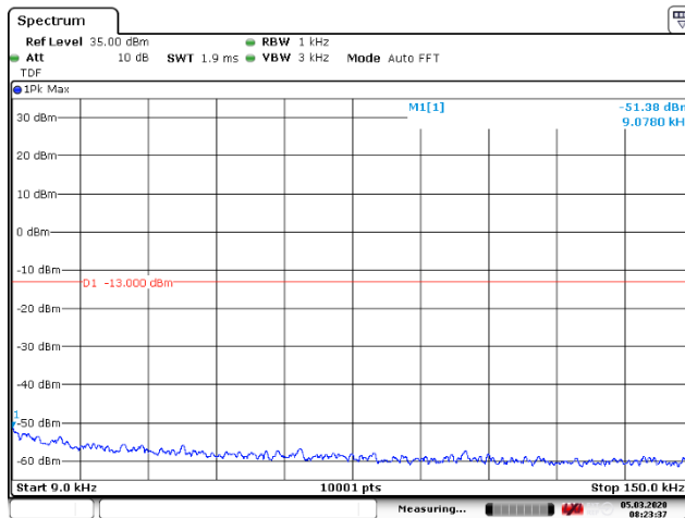
Figure 122: 9 – 150 kHz
