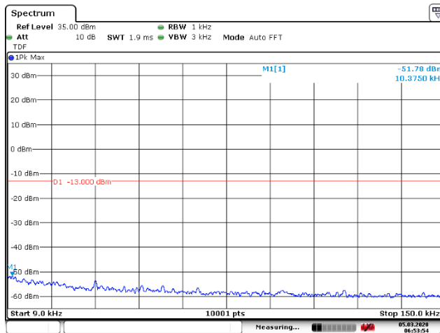
Figure 106: 9 – 150 kHz
