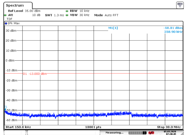
Figure 119: 150 kHz – 30 MHz
