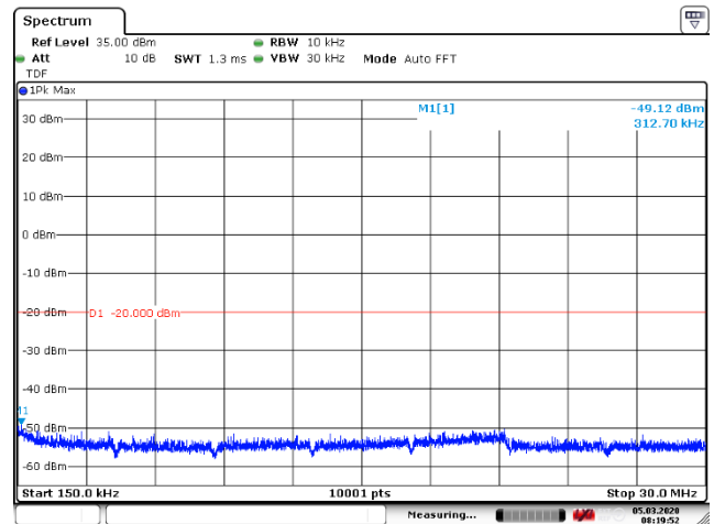
Figure 83: 150 kHz – 30 MHz
