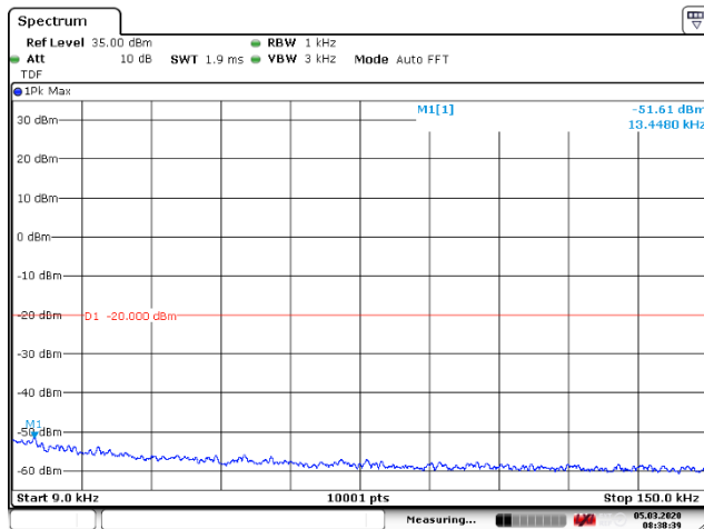
Figure 90: 9 – 150 kHz
