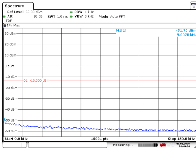
Figure 138: 9 – 150 kHz
