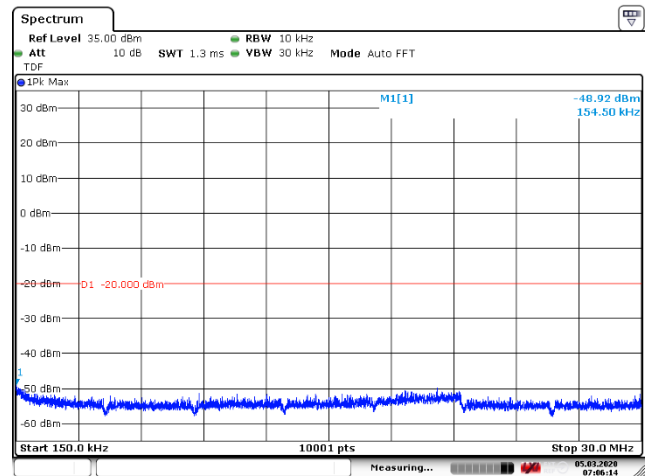
Figure 63: 150 kHz – 30 MHz
