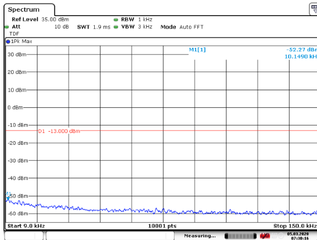
Figure 118: 9 – 150 kHz
