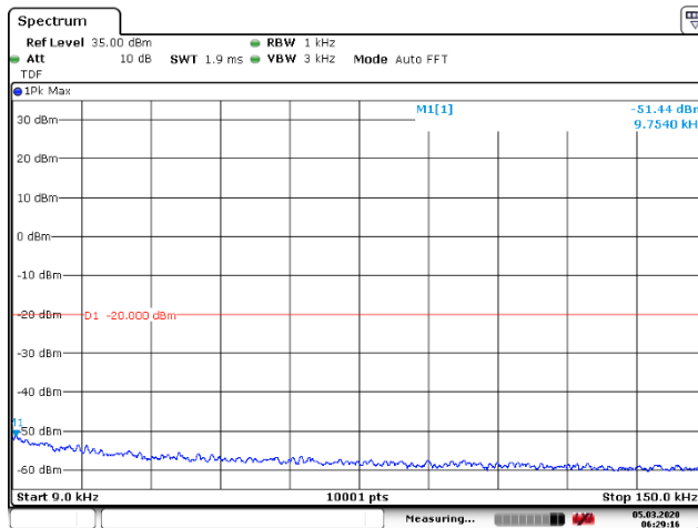
Figure 54: 9 – 150 kHz
