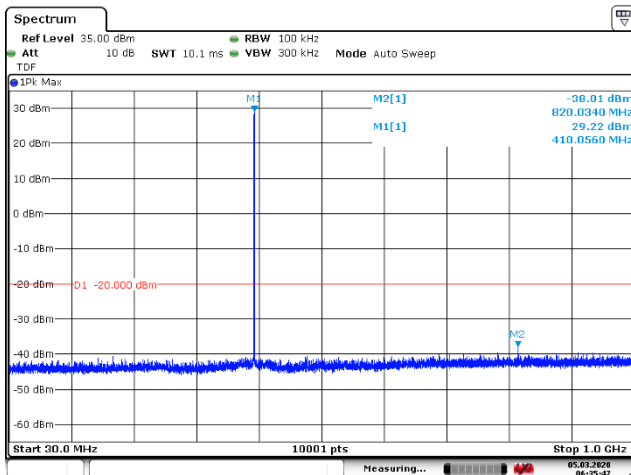
Figure 60: 30 – 1000 MHz
