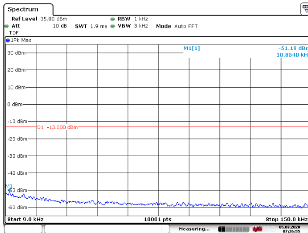
Figure 114: 9 – 150 kHz
