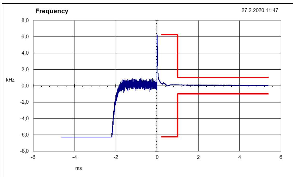
Figure 167: 469.5 MHz
