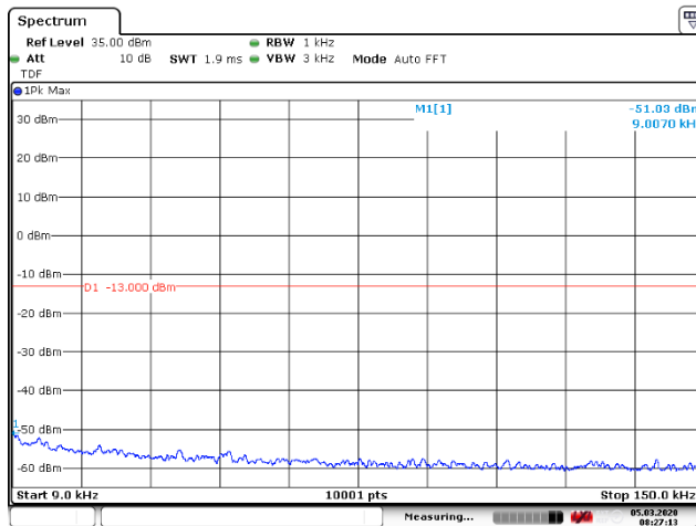
Figure 126: 9 – 150 kHz
