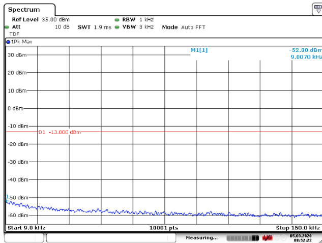
Figure 142: 9 – 150 kHz
