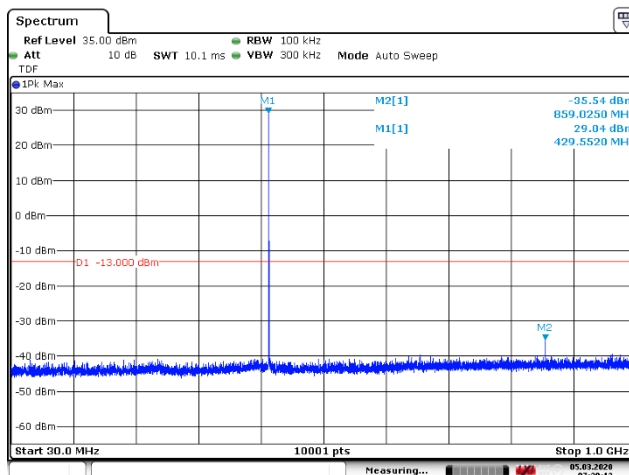
Figure 116: 30 – 1000 MHz
