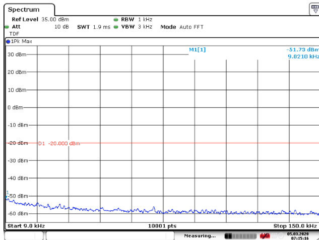
Figure 70: 9 – 150 kHz
