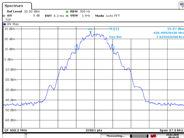
Figure 16: OBW (8 FSK, 12.5 kHz)
