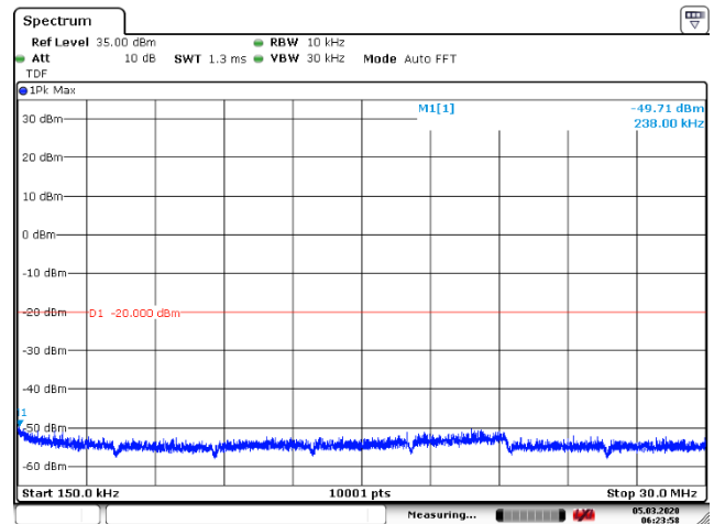
Figure 51: 150 kHz – 30 MHz
