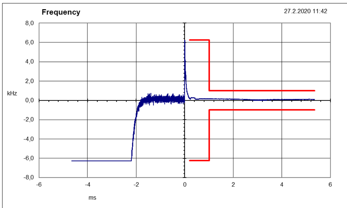
Figure 165: 429.5 MHz
