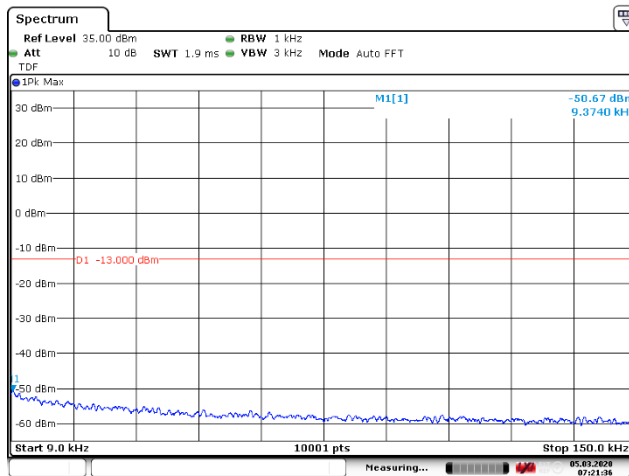
Figure 110: 9 – 150 kHz
