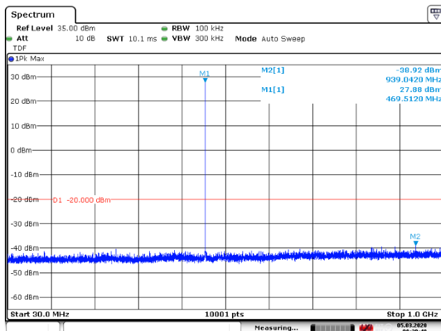
Figure 92: 30 – 1000 MHz
