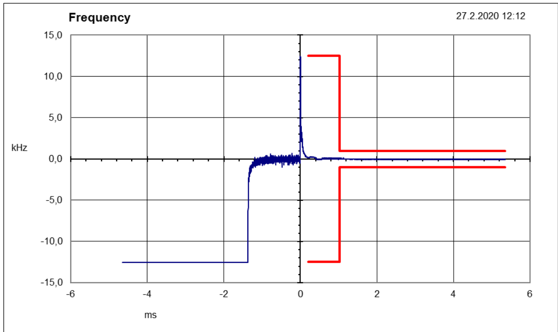
Figure 168: 410.0 MHz
