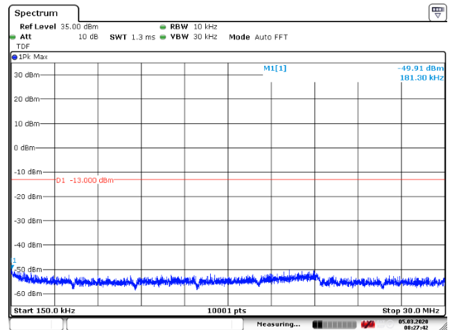
Figure 127: 150 kHz – 30 MHz
