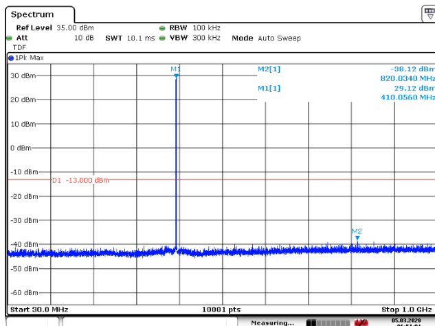
Figure 104: 30 – 1000 MHz
