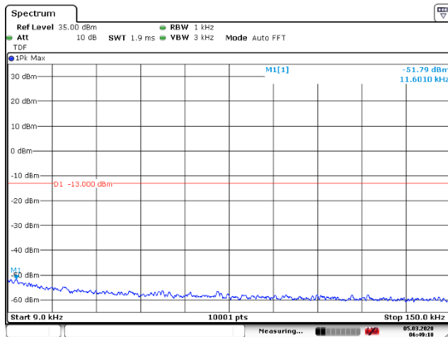
Figure 102: 9 – 150 kHz
