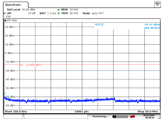
Figure 99: 150 kHz – 30 MHz
