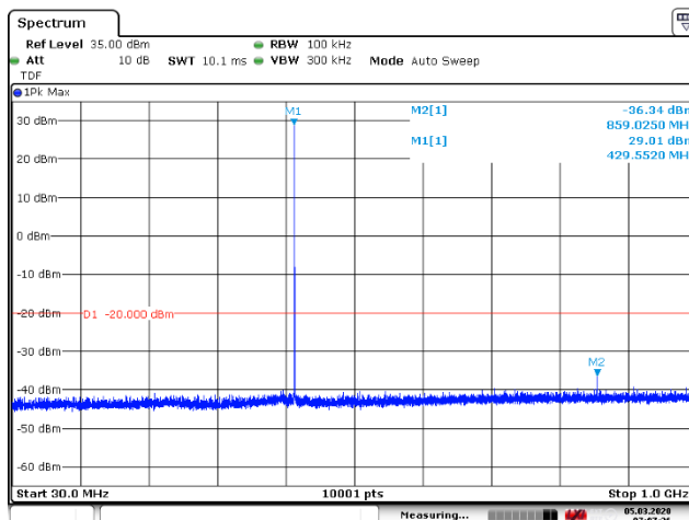
Figure 64: 30 – 1000 MHz
