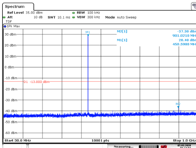
Figure 124: 30 – 1000 MHz
