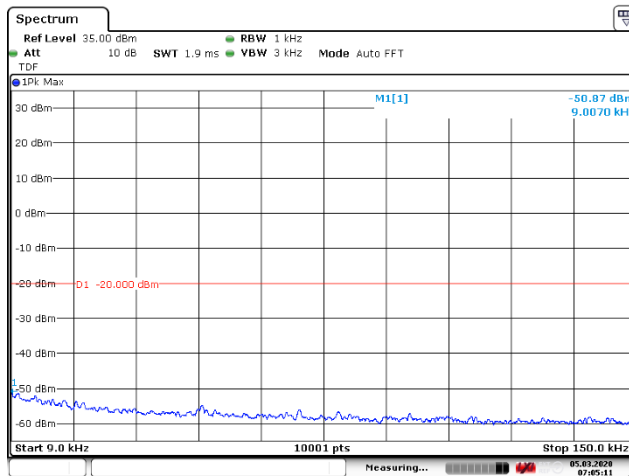
Figure 62: 9 – 150 kHz
