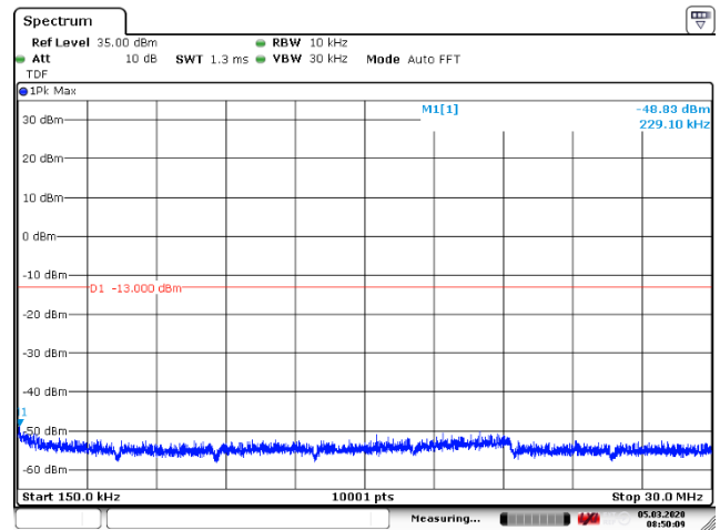
Figure 139: 150 kHz – 30 MHz
