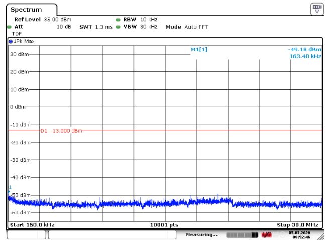
Figure 143: 150 kHz – 30 MHz
