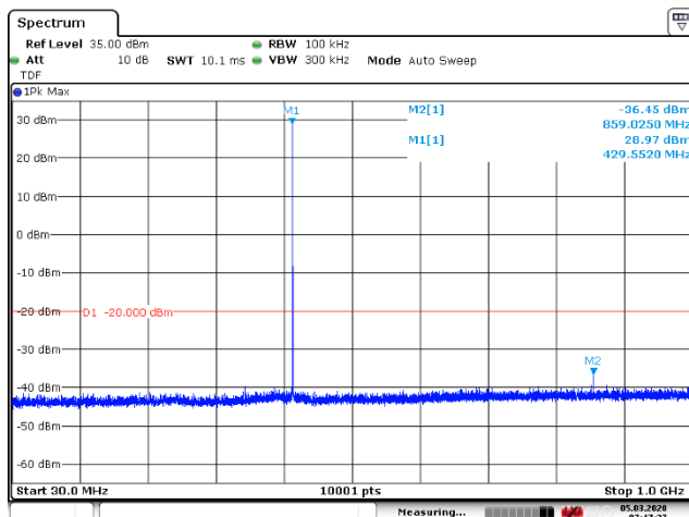
Figure 72: 30 – 1000 MHz
