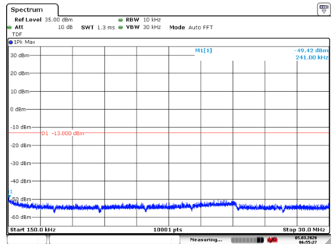
Figure 107: 150 kHz – 30 MHz
