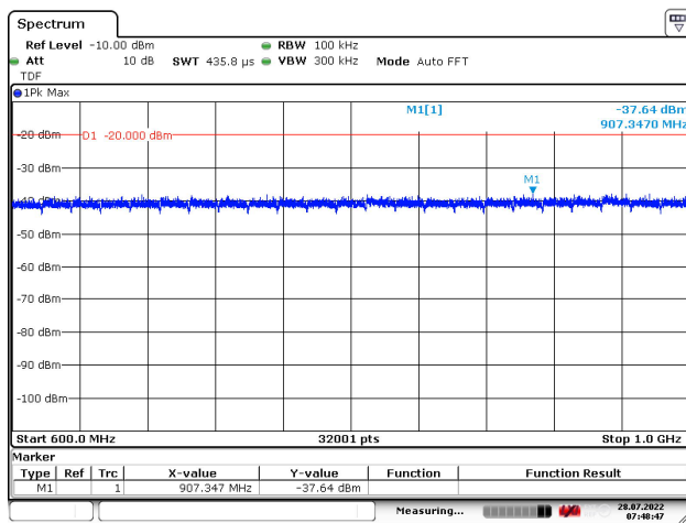
Figure 54: 600 – 1000 MHz
