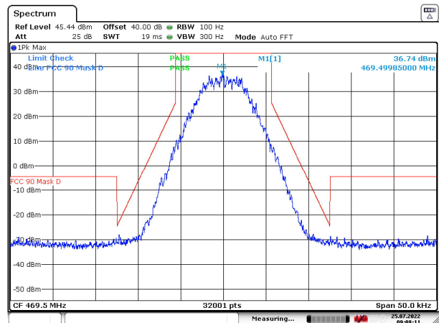
Figure 9: 469.5 MHz
