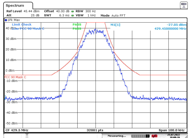
Figure 27: 429.5 MHz
