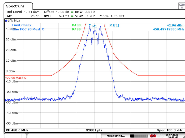
Figure 40: 450.5 MHz
