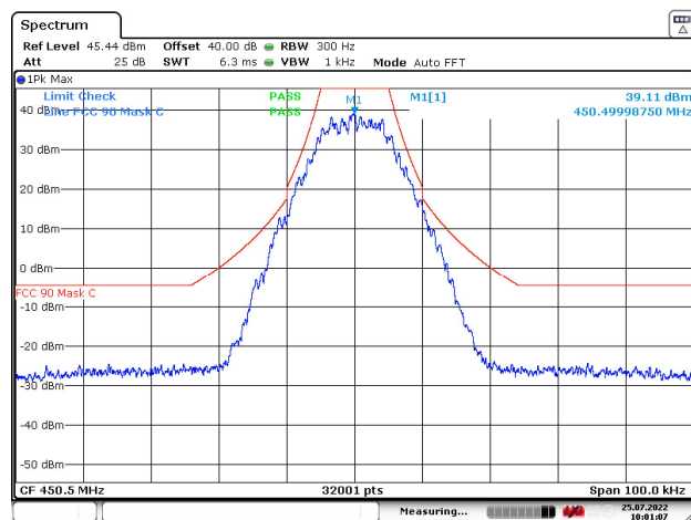
Figure 28: 450.5 MHz
