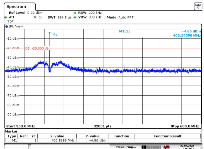
Figure 53: 350 – 600 MHz
