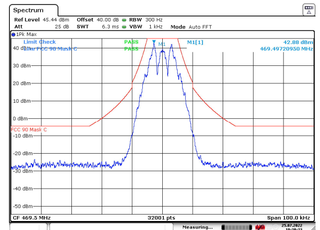
Figure 41: 469.5 MHz
