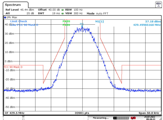
Figure 7: 429.5 MHz
