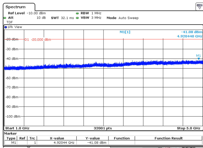
Figure 55: 1000 – 5000 MHz
