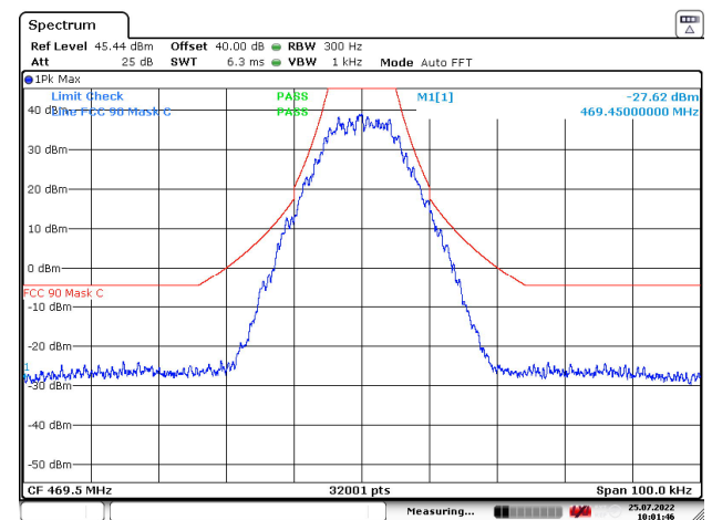
Figure 29: 469.5 MHz
