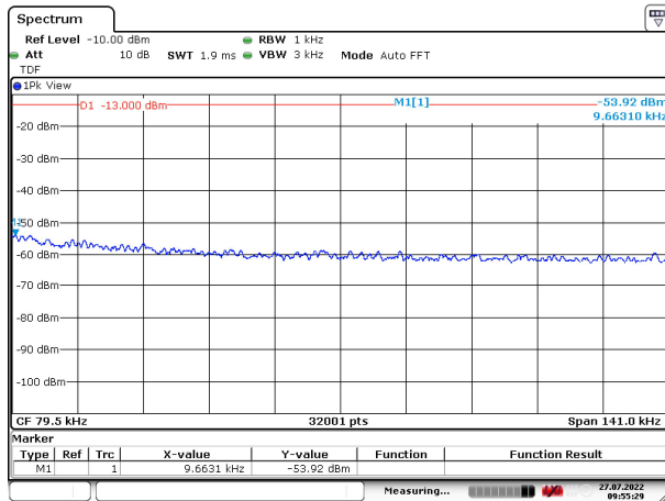
Figure 260: 9 – 150 kHz
