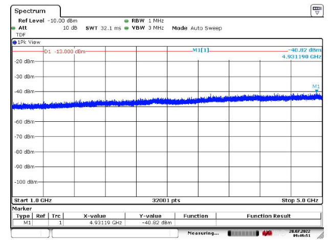
Figure 289: 1000 – 5000 MHz
