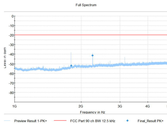
Figure 334: 8FSK, Ch Width 12.5kHz, 450.5 MHz, X
