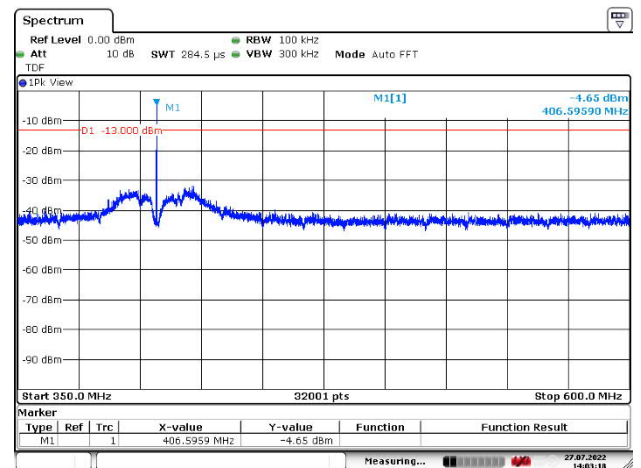
Figure 293: 350 – 600 MHz
