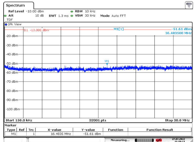
Figure 267: 150 kHz – 30 MHz
