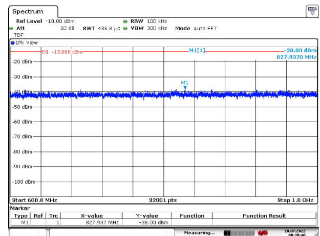
Figure 270: 600 – 1000 MHz
