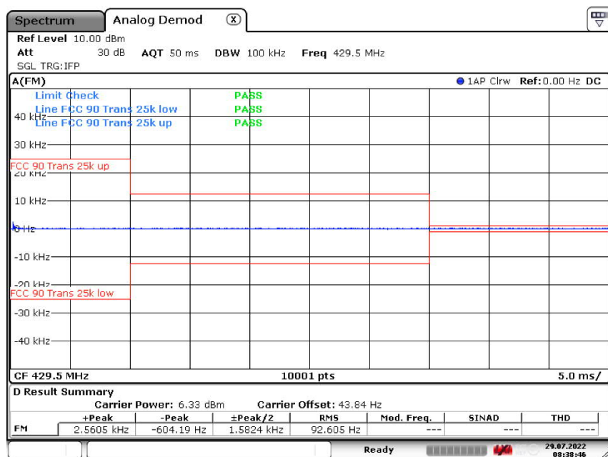
Figure 360: 429.5 MHz
