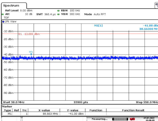
Figure 286: 30 – 350 MHz
