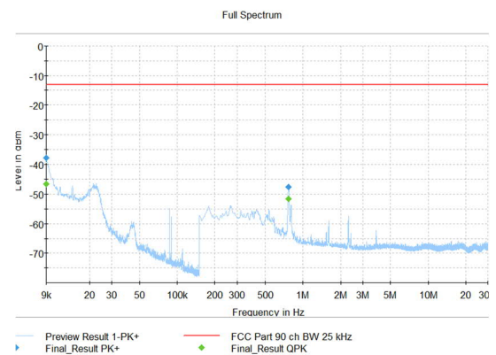
Figure 317: 8FSK, Ch Width 25kHz, 469.5 MHz, X
