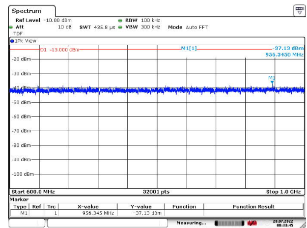
Figure 294: 600 – 1000 MHz
