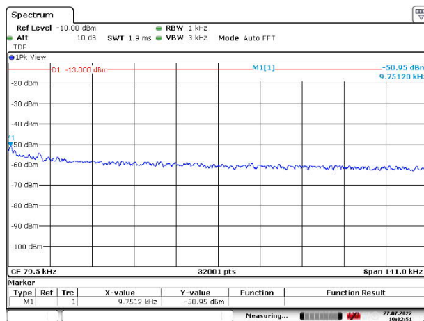
Figure 308: 9 – 150 kHz
