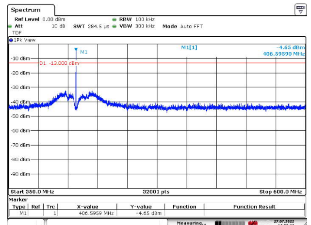
Figure 269: 350 – 600 MHz
