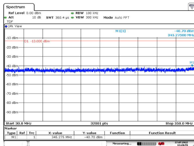
Figure 274: 30 – 350 MHz
