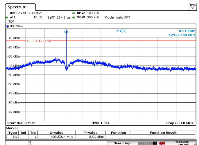
Figure 275: 350 – 600 MHz
