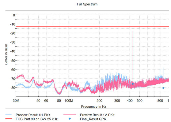
Figure 346: GMSK 9600bps, Ch Width 25kHz, 429.5 MHz, X
