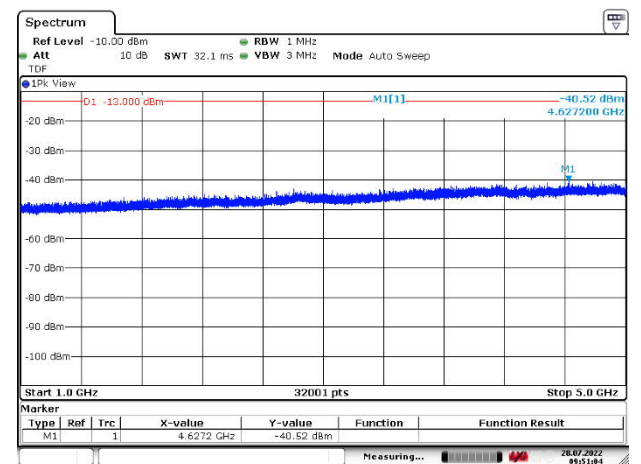
Figure 295: 1000 – 5000 MHz
