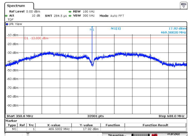
Figure 311: 350 – 600 MHz
