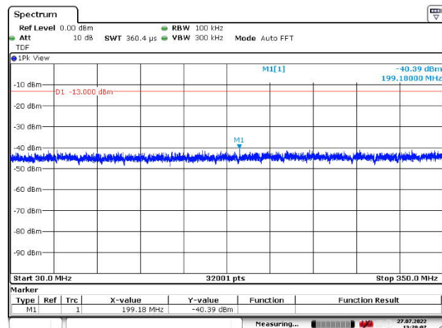
Figure 268: 30 – 350 MHz
