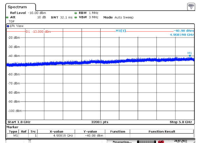
Figure 271: 1000 – 5000 MHz
