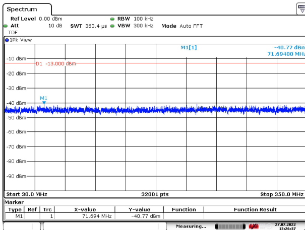
Figure 262: 30 – 350 MHz
