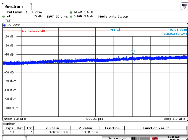
Figure 265: 1000 – 5000 MHz
