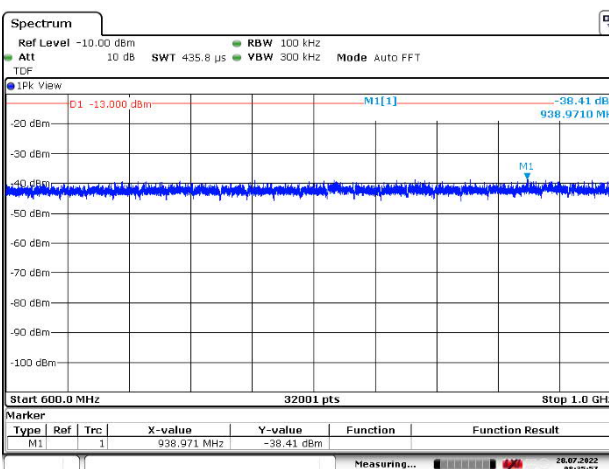
Figure 312: 600 – 1000 MHz
