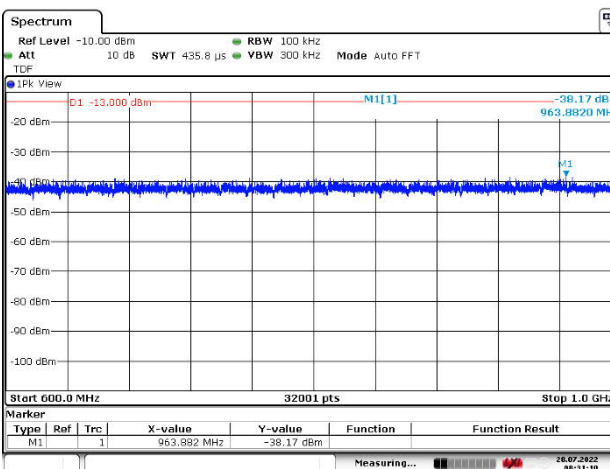
Figure 288: 600 – 1000 MHz
