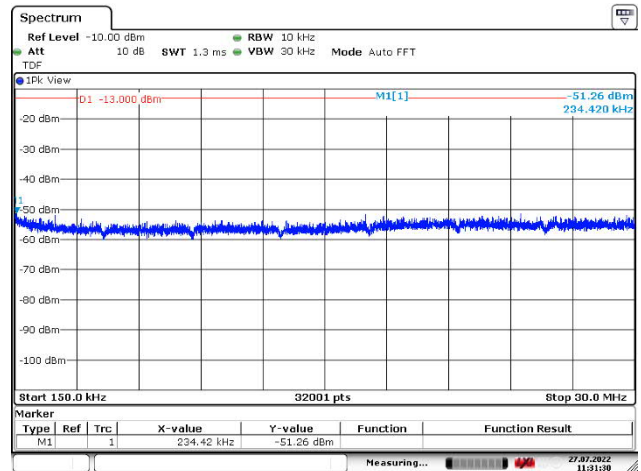
Figure 291: 150 kHz – 30 MHz
