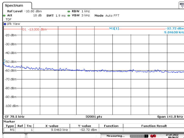
Figure 266: 9 – 150 kHz
