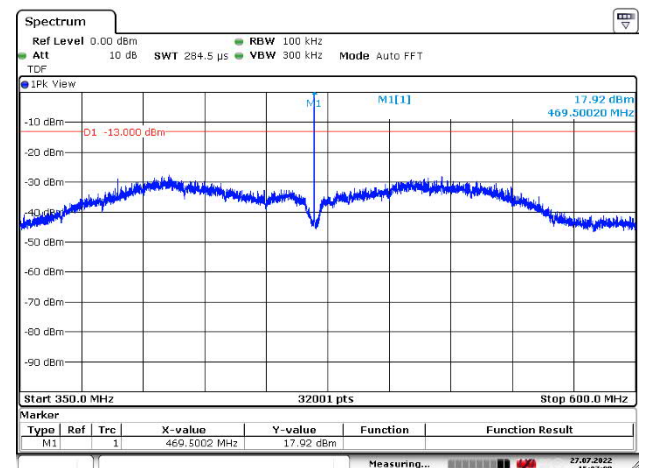
Figure 287: 350 – 600 MHz
