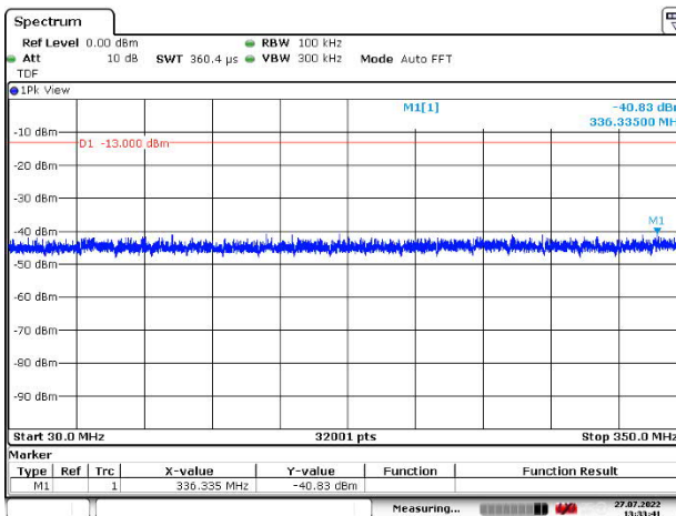
Figure 310: 30 – 350 MHz
