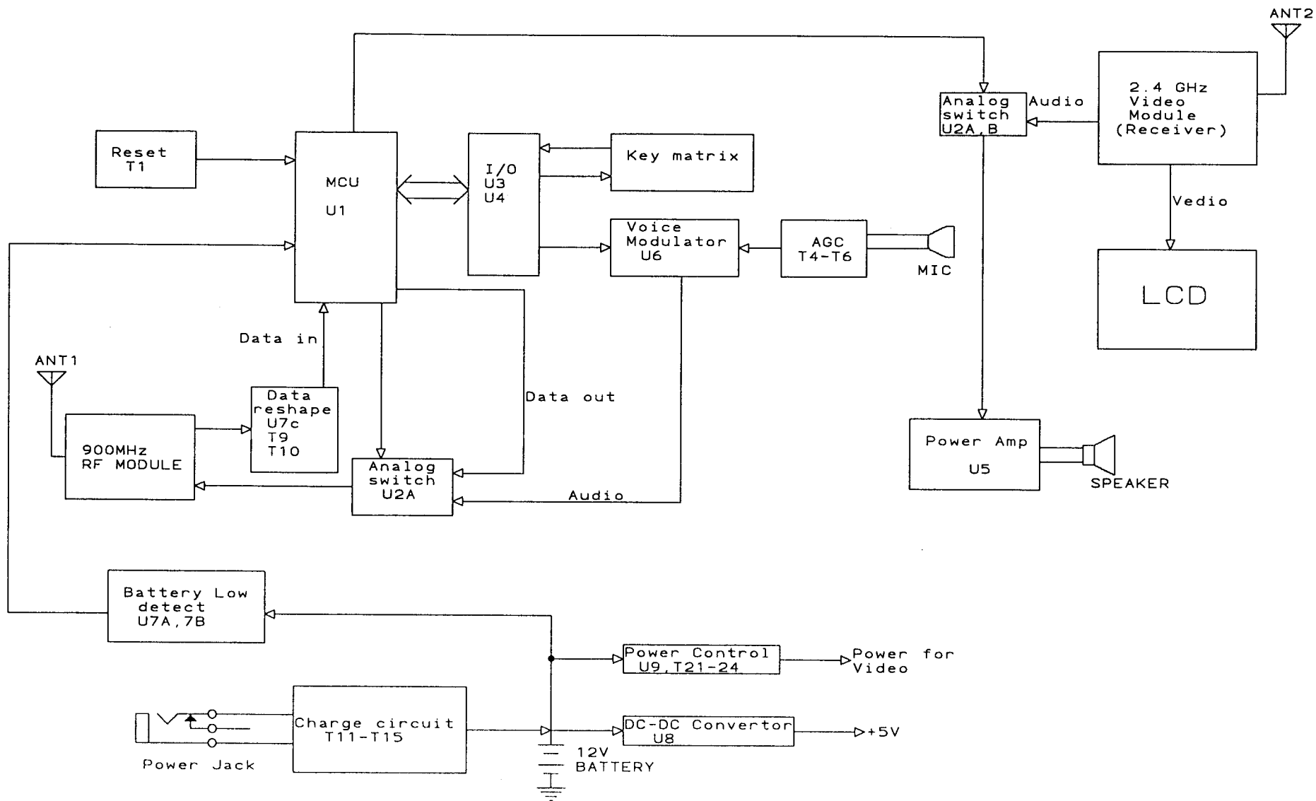
REMOTE CONTROL BLOCK DIAGRAM
