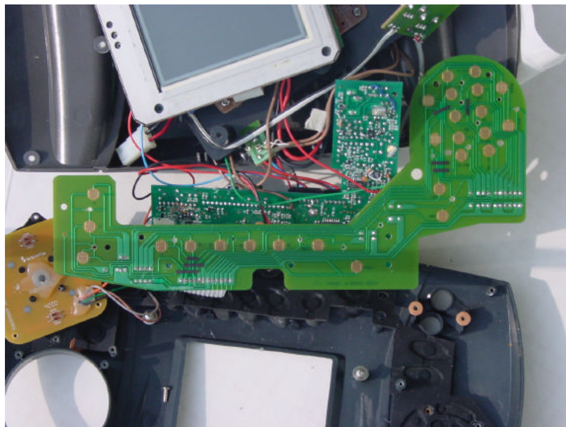
Keypad (Solder Side)
