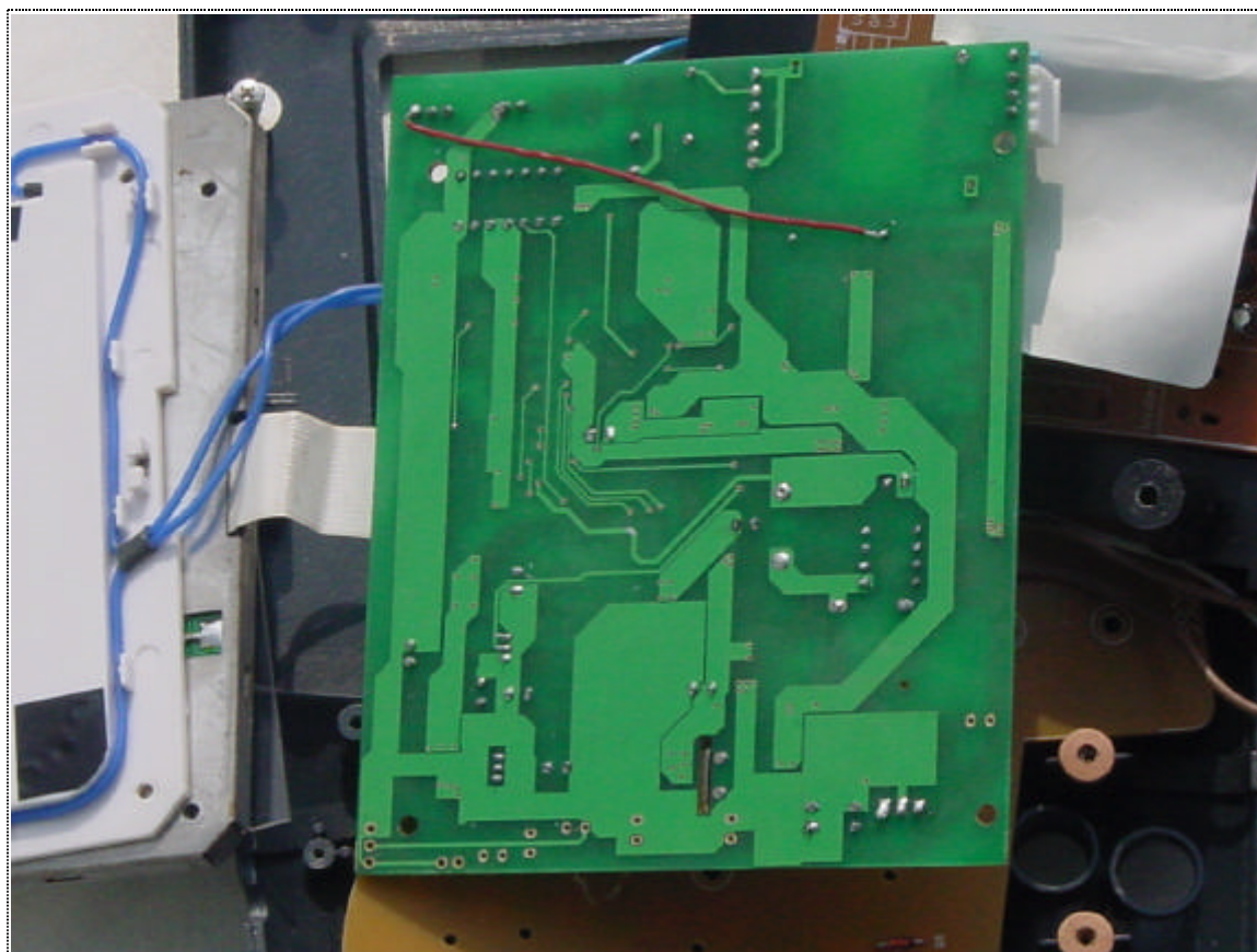
LCD Control Board (Solder Side)
