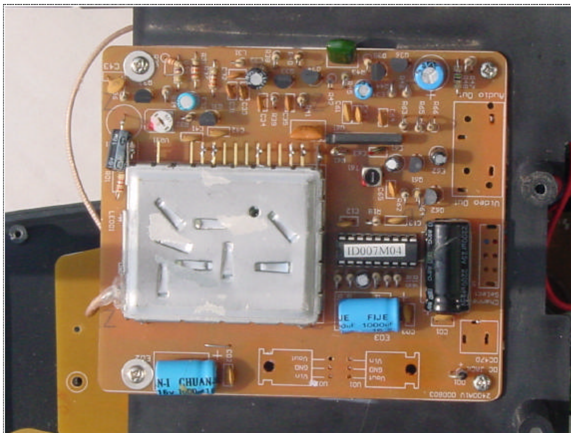
RF Module – Audio &amp; Video (Remote Controller, Component Side)
