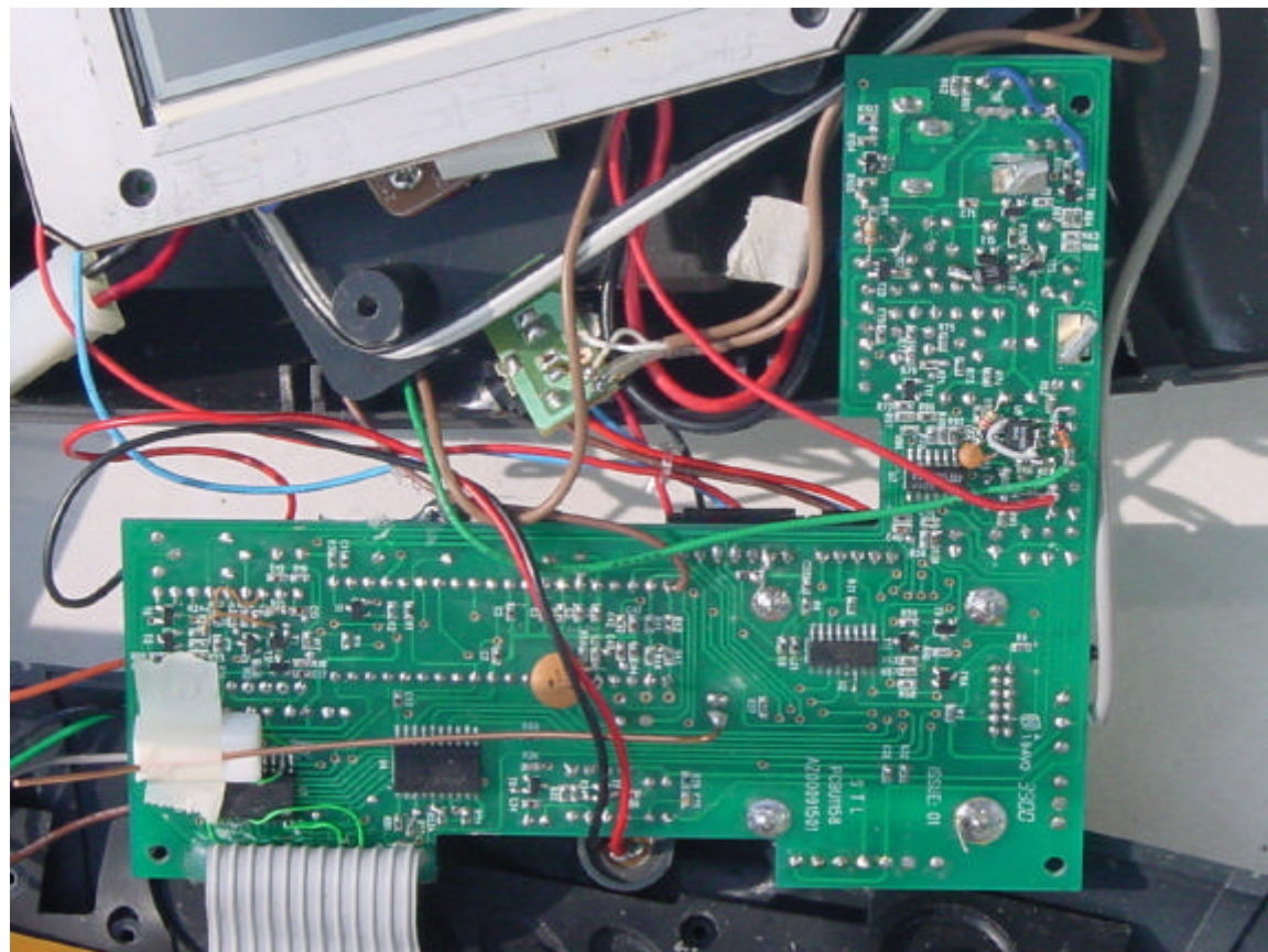
RF Module – Data &amp; Voice (Remote Controller, Solder Side)
