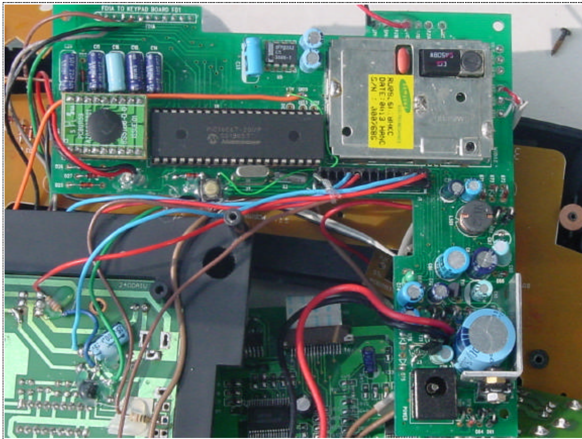
RF Module – Data &amp; Voice (Remote Controller, Component Side)
