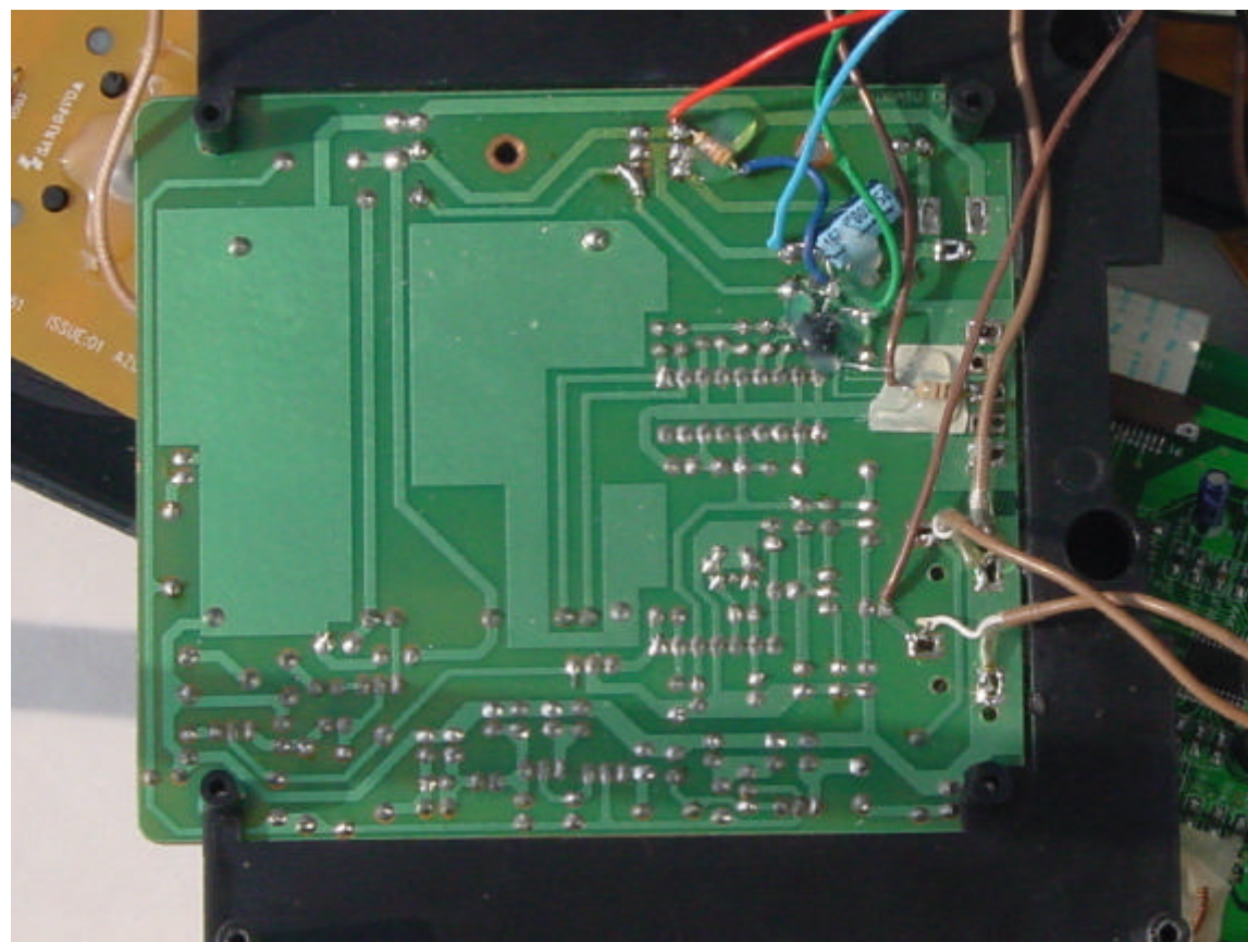
RF Module – Audio &amp; Video (Remote Controller, Solder Side)
