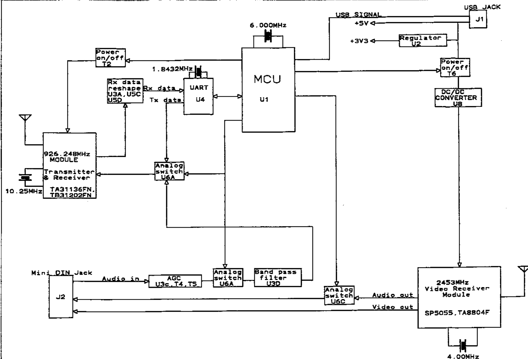
SI983 BLOCK DIAGRAM
