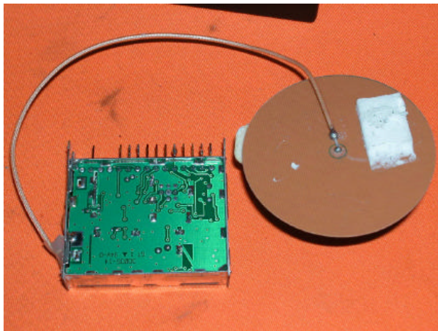
Internal Photo – 8 (900MHZ RF Module)
