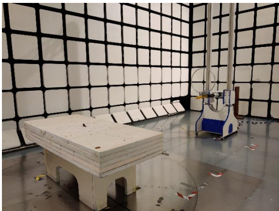
Radio-frequency radiated emissions (9 kHz - 30 MHz).
