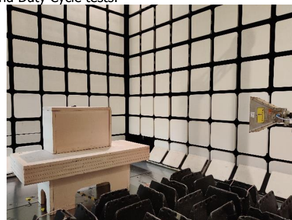
Radio-frequency radiated emissions (1 GHz – 6 GHz)
