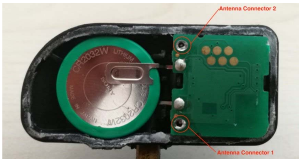
(7) EUT Photo
