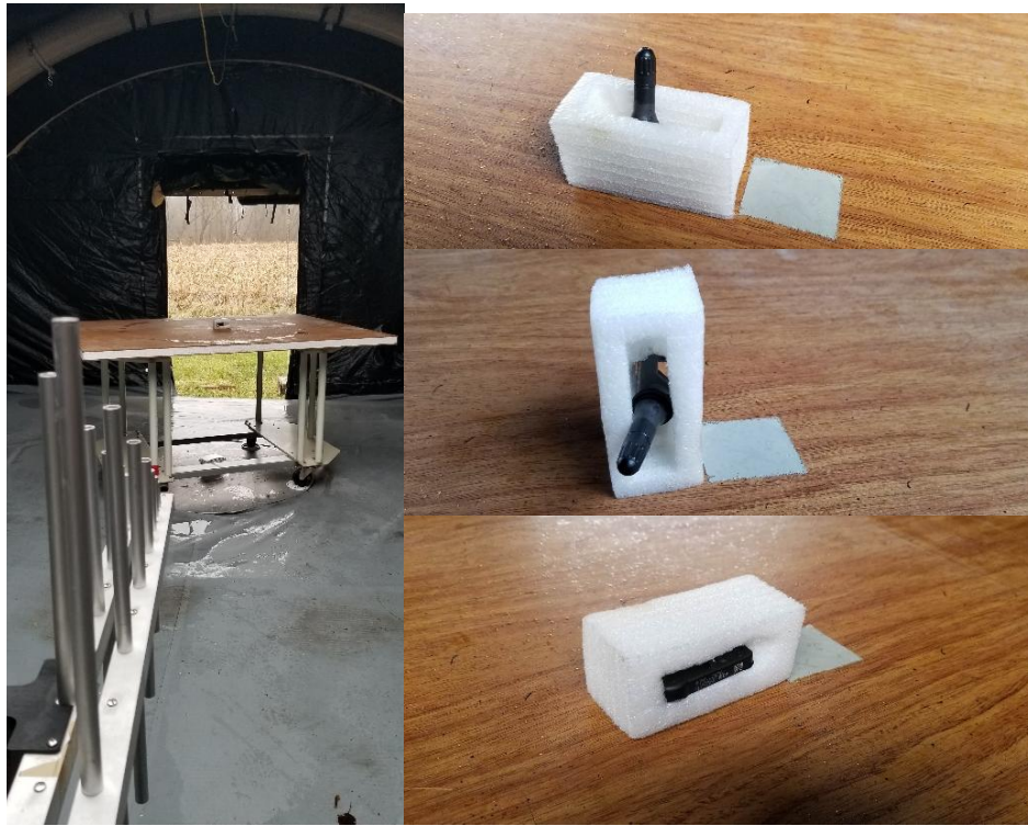
Figure 4: Radiated Emissions Test Setup Photograph(s).
