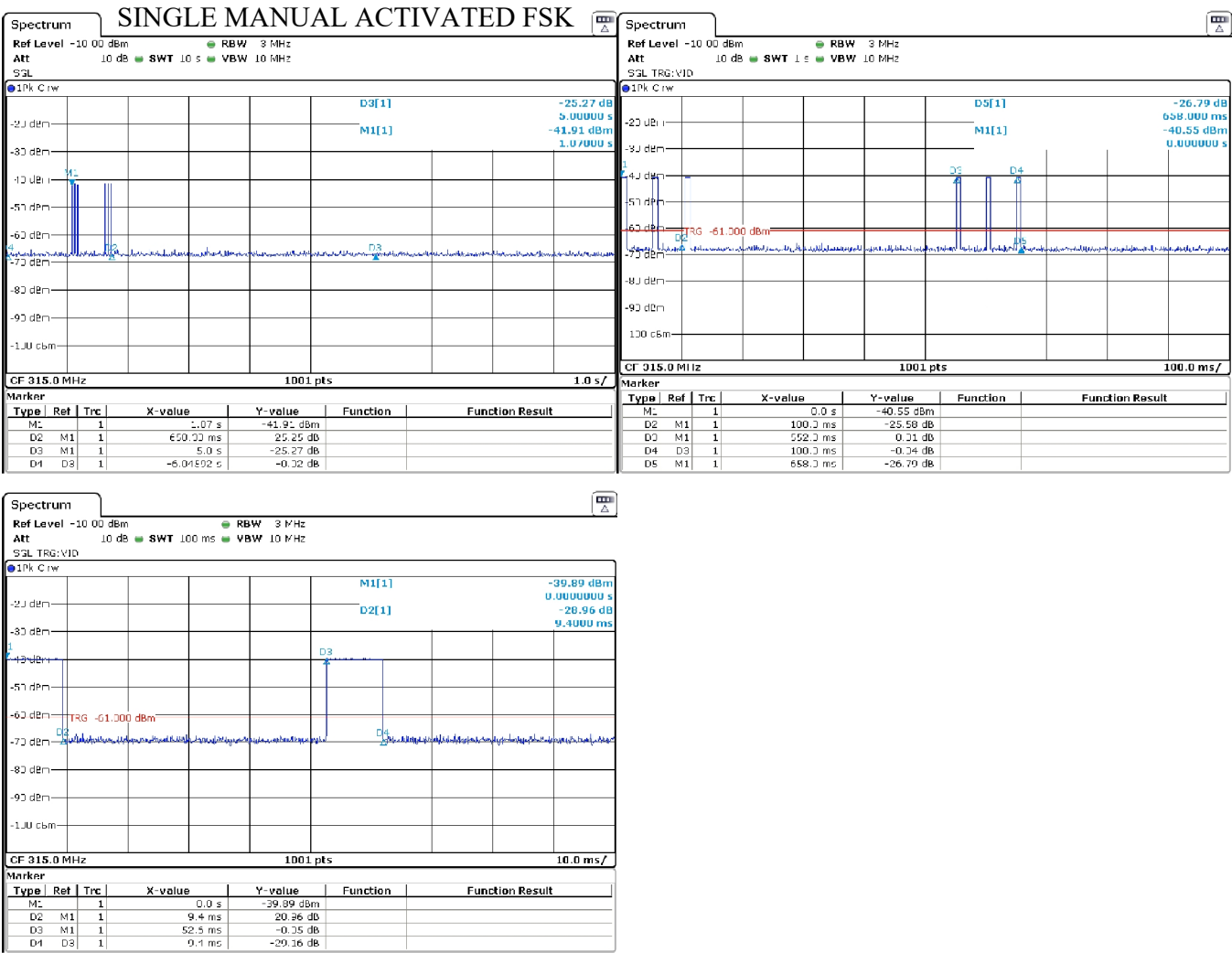
Figure 5(c): Fundamental Emission Pulsed Operation.
