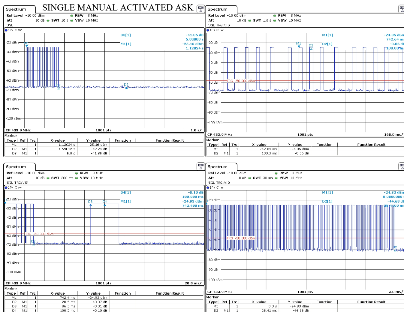
Figure 5(e): Fundamental Emission Pulsed Operation.
