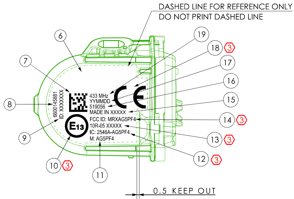
Bottom View
