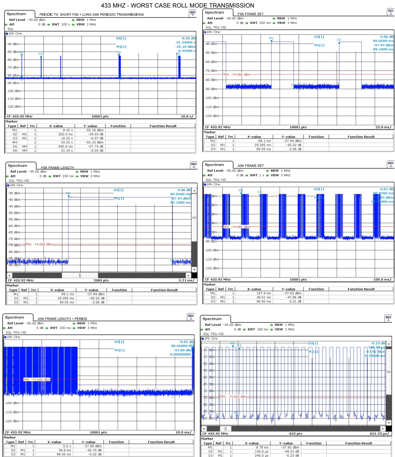
Figure 5(d): Fundamental Emission Pulsed Operation.
