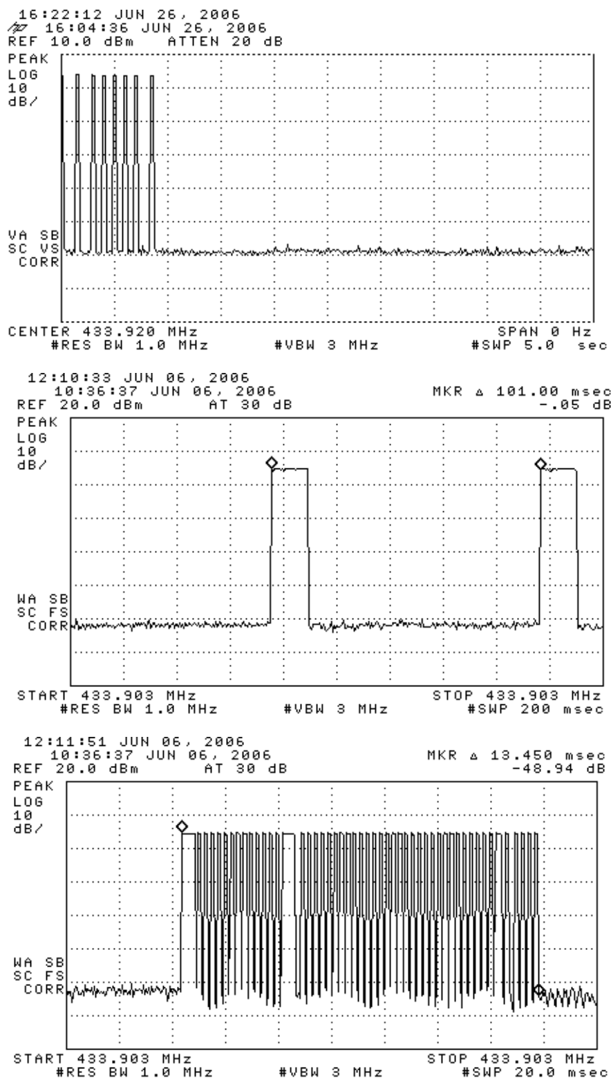
Figure 6.1(a). Transmissions modulation characteristics: (top) complete transmission, (center) expanded period, (bottom) expanded word.
