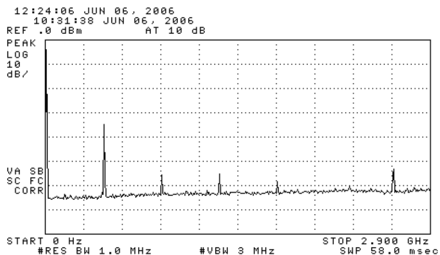
Figure 6.2(a). Emission spectrum of the DUT (7653494 pulsed emission). The amplitudes are only indicative (not calibrated).
