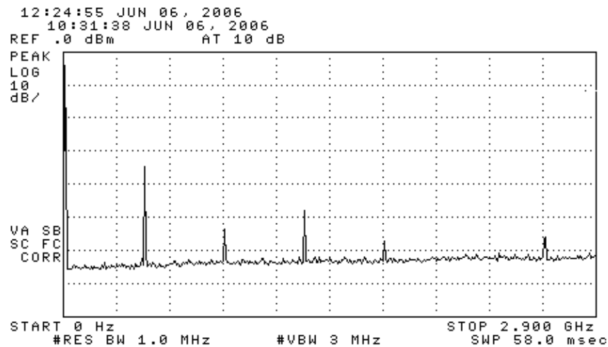
Figure 6.2(b). Emission spectrum of the DUT (7694420 pulsed emission). The amplitudes are only indicative (not calibrated).
