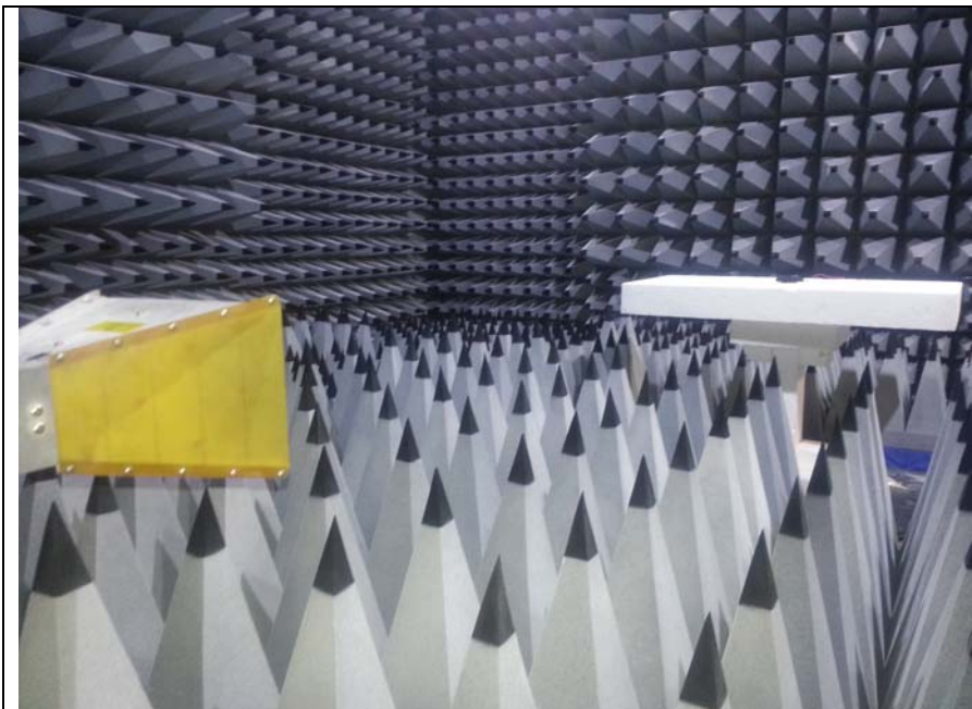
Fig 4 Test setup Rad Emissions Receive mode >1GHz
