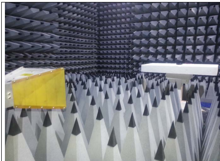
Fig 2 Test setup 1GHz -4.5 GHz Rad Emissions
