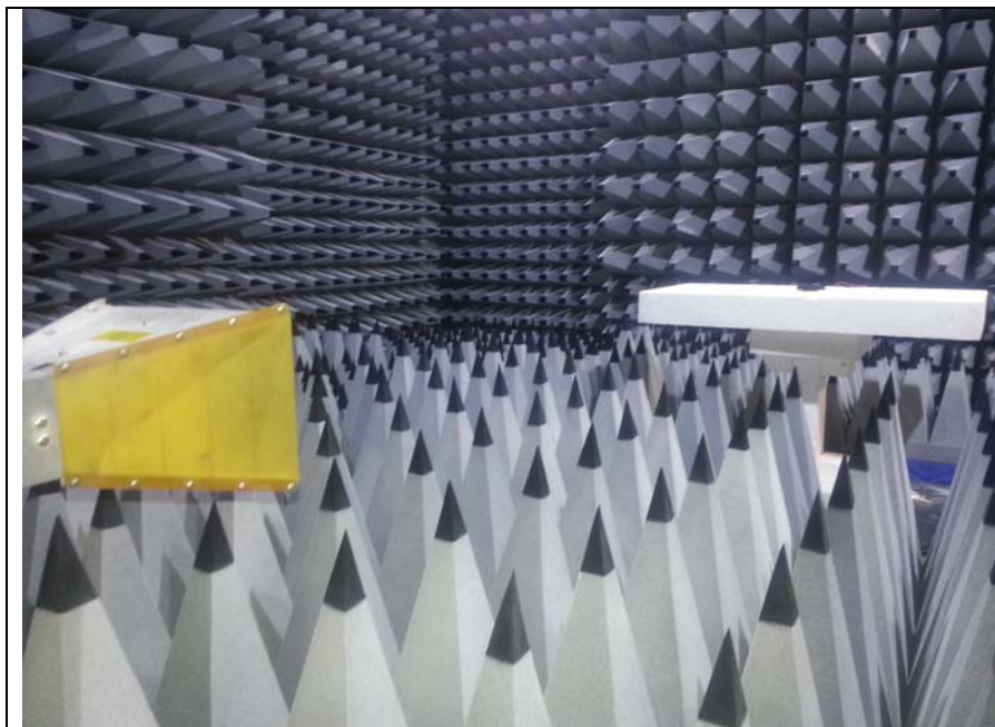
Fig 2 Test setup 1GHz -4.5 GHz Rad Emissions Transmit mode
