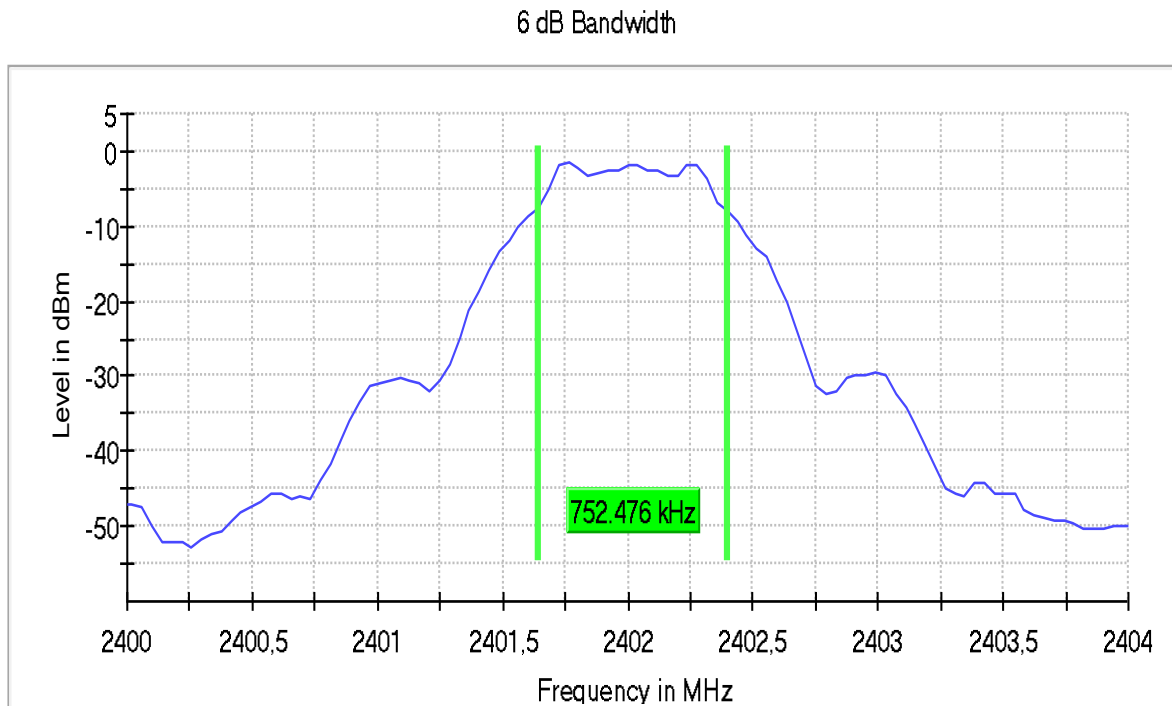
Plot 1: Mode 1, DTS Bandwidth, low channel
