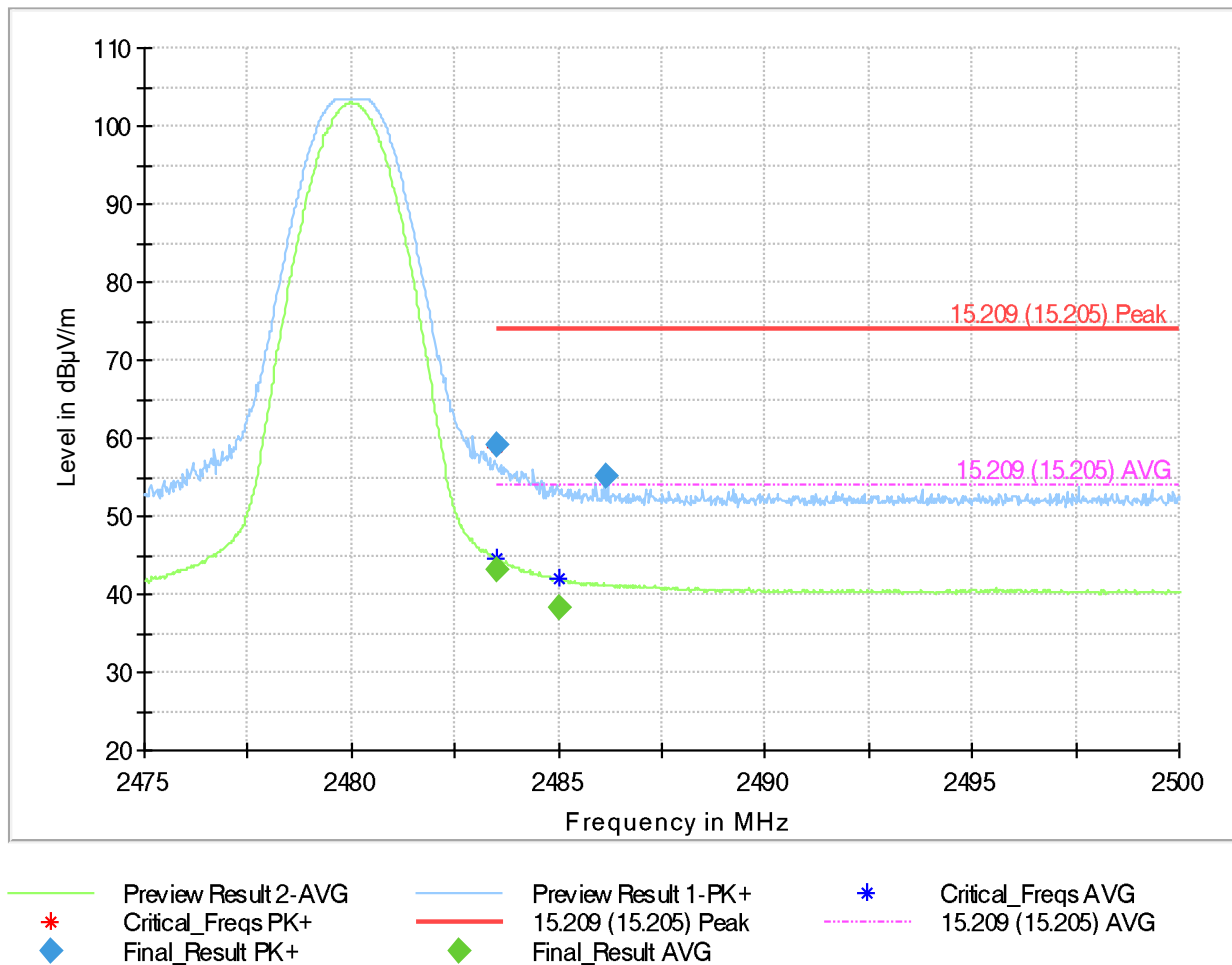
Plot 16: Mode 1, BEC, high channel
