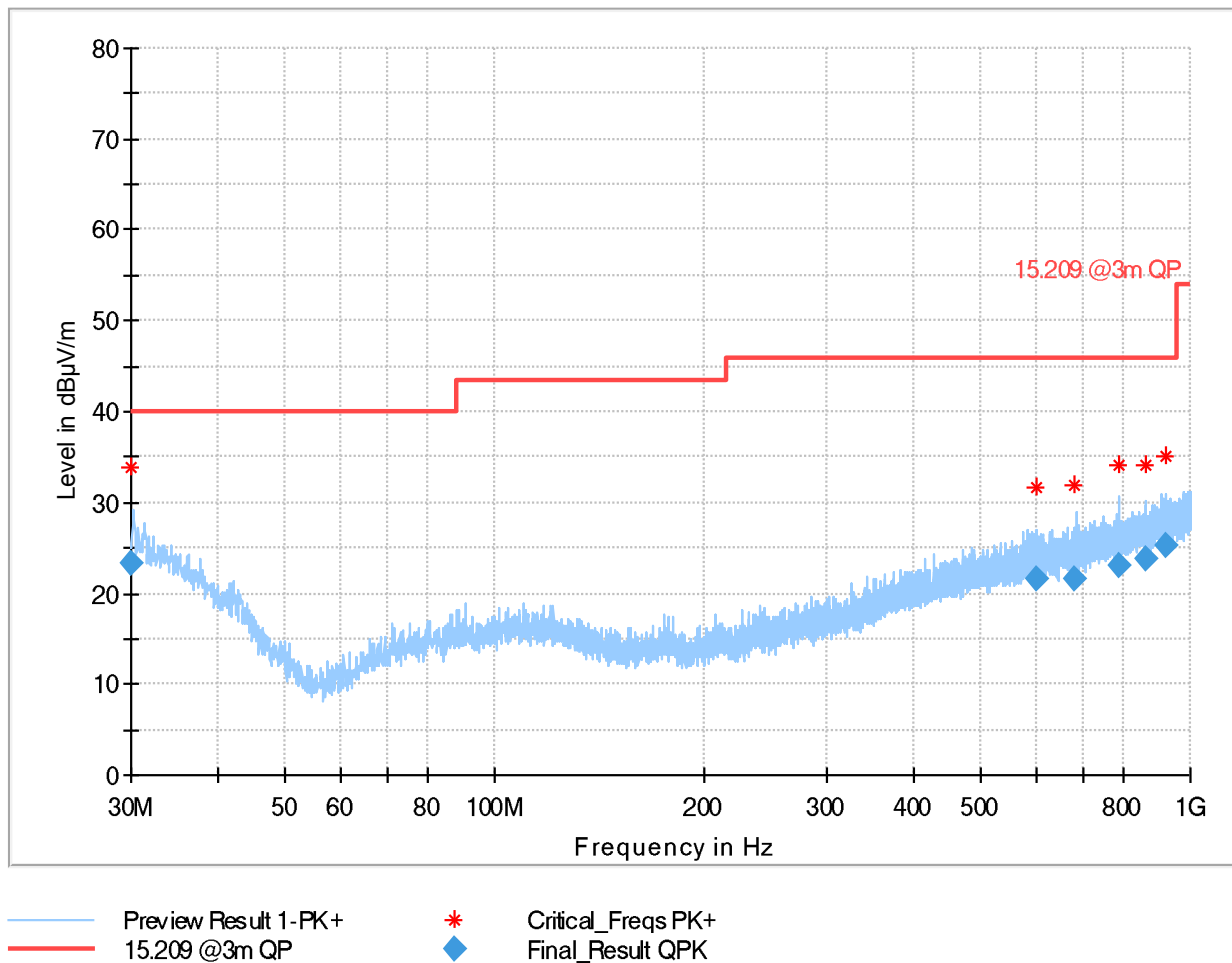
Plot 24: Mode 1, RSE 30 MHz – 1 GHz, mid channel, horizontal / vertical polarisation
