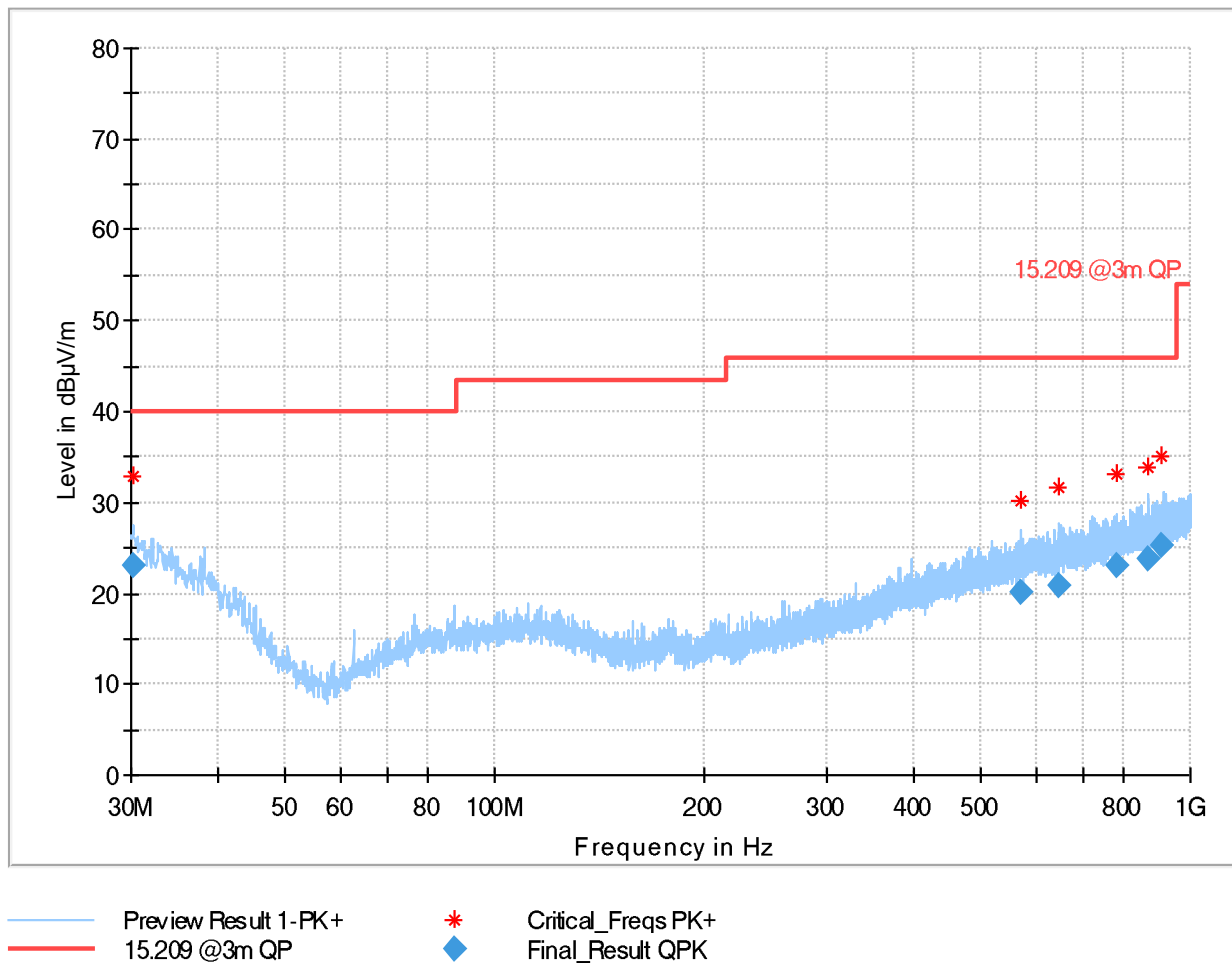
Plot 25: Mode 1, RSE 30 MHz – 1 GHz, high channel, horizontal / vertical polarisation
