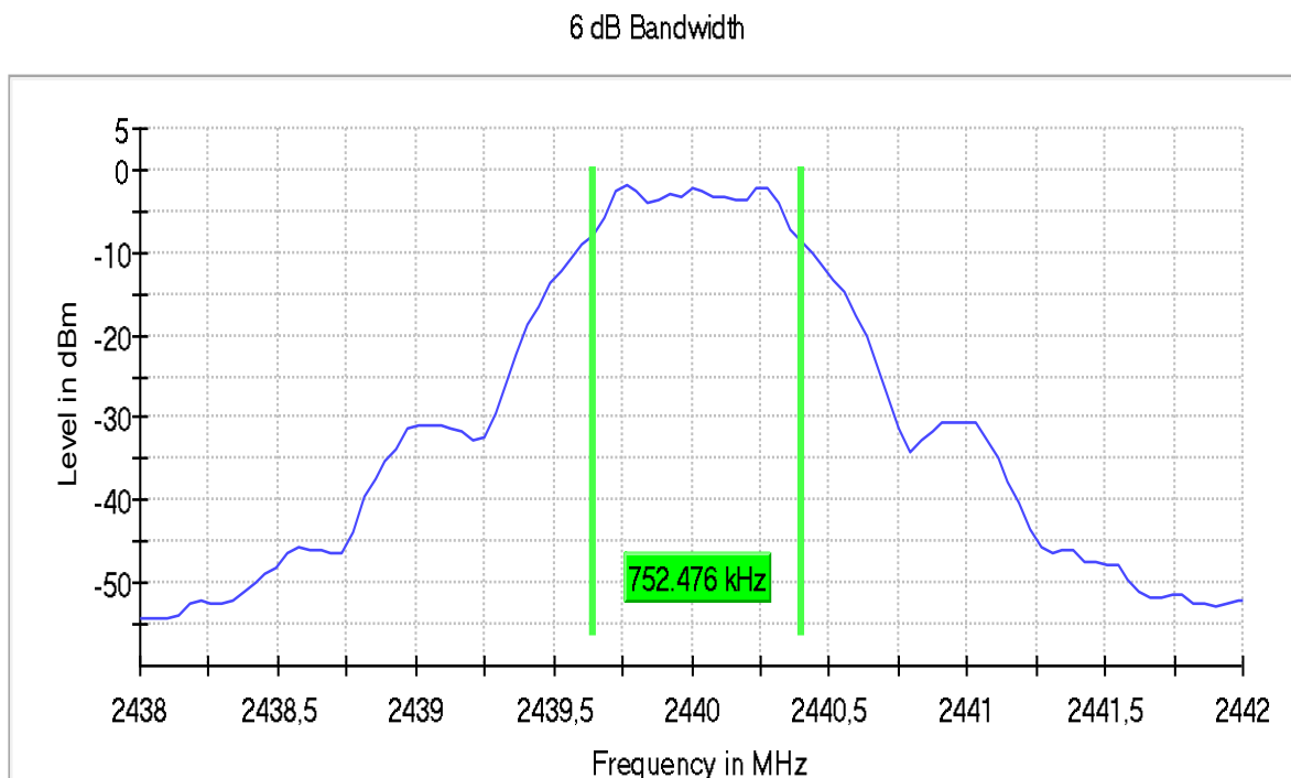
Plot 2: Mode 1, DTS Bandwidth, mid channel
