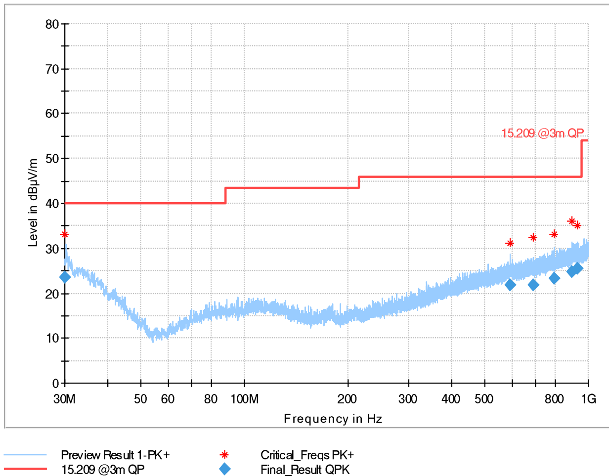
Plot 23: Mode 1, RSE 30 MHz – 1 GHz, low channel, horizontal / vertical polarisation
