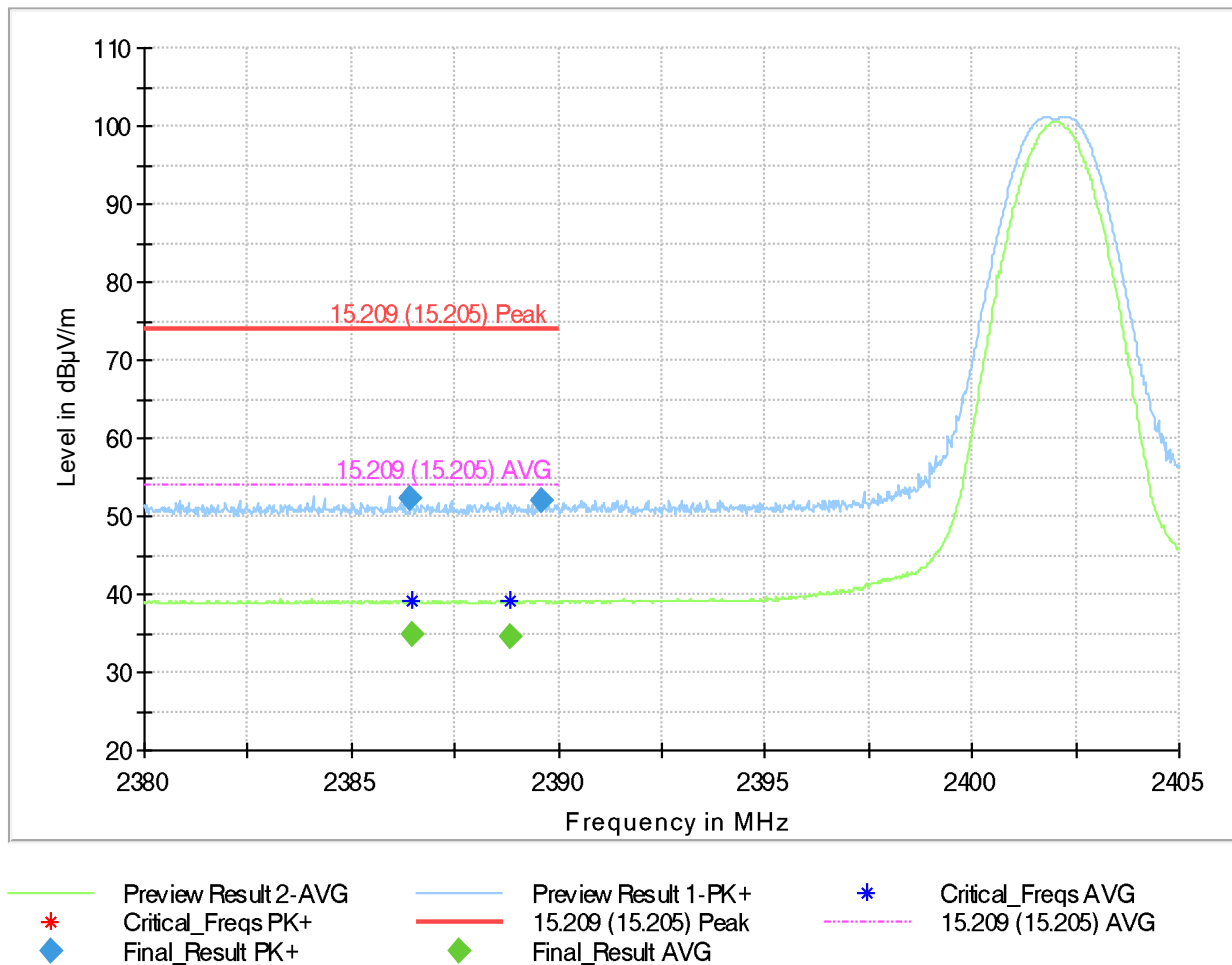
Plot 15: Mode 1, BEC, low channel
