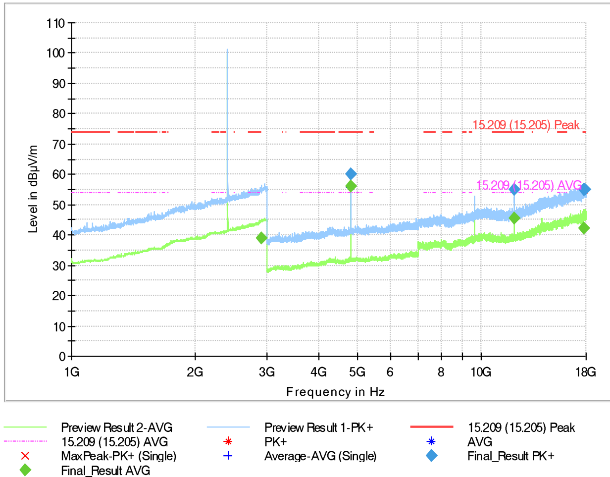
Plot 26: Mode 1, RSE 1 GHz – 18 GHz, low channel, horizontal / vertical polarisation
