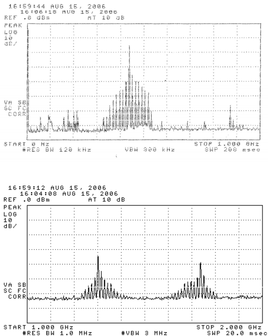
Figure 6.2. Emission spectrum of the DUT (pulsed emission). The amplitudes are only indicative (not calibrated).
