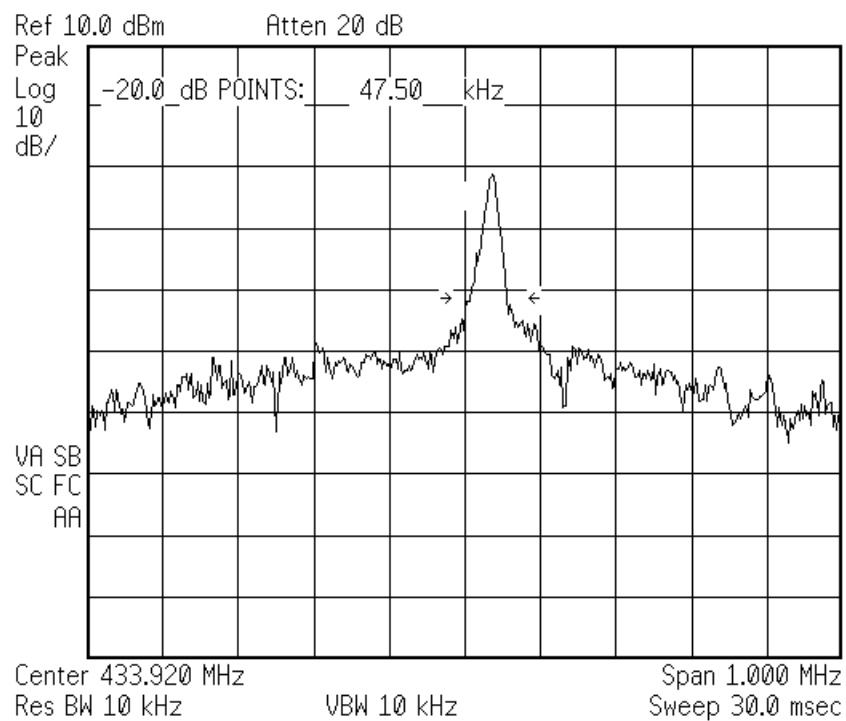
Figure 6.3. Measured bandwidth of the DUT (pulsed emission).
