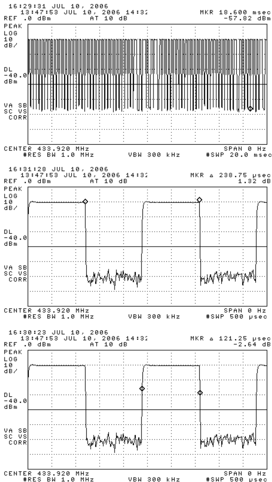
Figure 6.1(b). Transmissions modulation characteristics: (top) zoomed word, (center) Manchester period, (bottom) Manchester pulse width.
