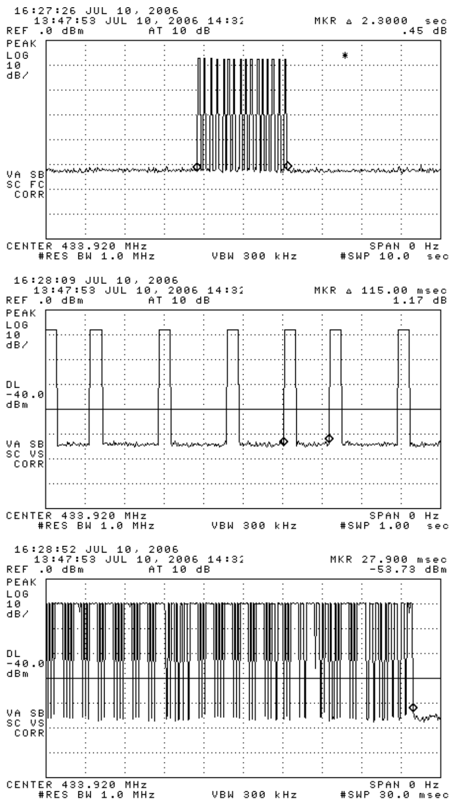
Figure 6.1(a). Transmissions modulation characteristics: (top) LF act. transmission, (center) minimum word separation, (bottom) expanded word.
