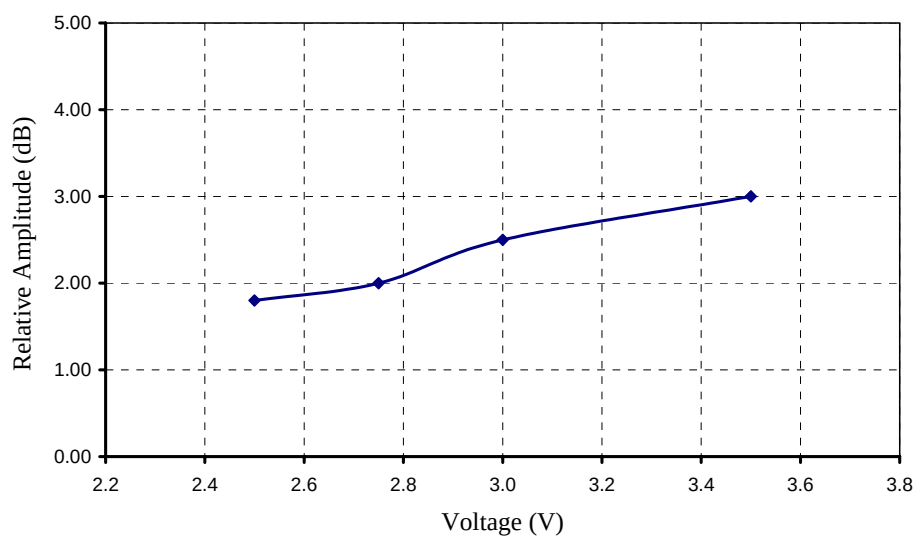
Figure 6.4. Relative emissions at 433.92 MHz vs. supply voltage. (cw emission)
